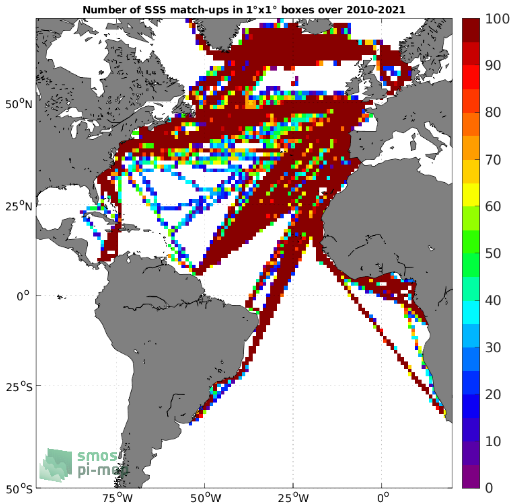
Figure 4: Number of SSS match-ups between TSG (LEGOS-DM) SSS and the SMOS SSS L3 v335 - 10 Days - 25 km (CATDS-CPDC) SSS product for the Atlantic Ocean Pi-MEP region over 1°x1° boxes and for the full satellite product period.
