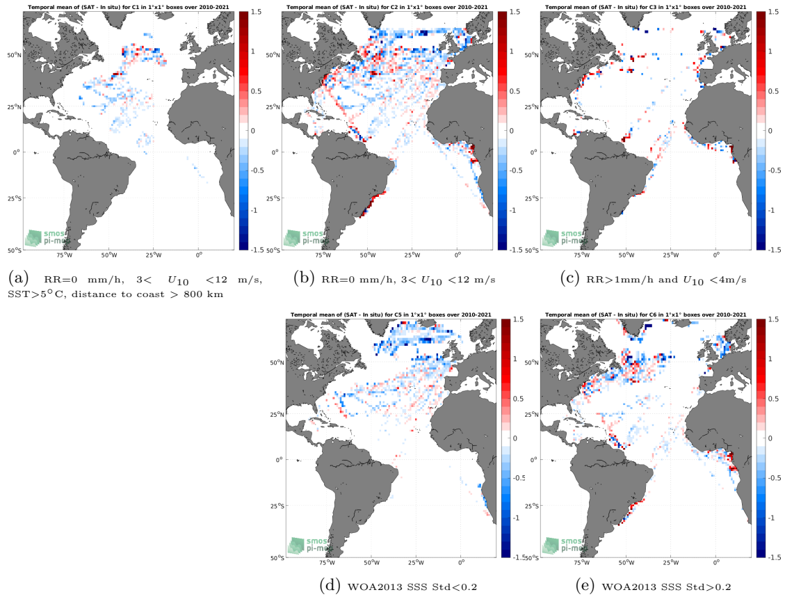
Figure 12: Temporal mean gridded over spatial boxes of size 1^\circ \times 1^\circ of \Delta\text{SSS} (SMOS SSS L3 v335 - 10 Days - 25 km (CATDS-CPDC) - TSG (LEGOS-DM)) for 5 different subdatasets corresponding to:RR=0 mm/h, 3 < U_{10} < 12 m/s, SST >5^\circ\text{C} , distance to coast > 800 km (a), RR=0 mm/h, 3 < U_{10} < 12 m/s (b), RR >1 mm/h and U_{10} < 4 m/s (c), WOA2013 SSS Std <0.2 (d), WOA2013 SSS Std >0.2 (e).
