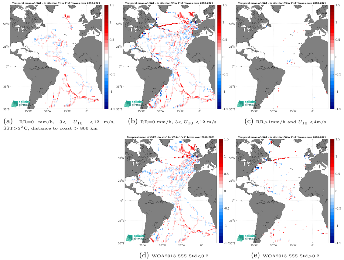
Figure 12: Temporal mean gridded over spatial boxes of size 1^\circ \times 1^\circ of \Delta\text{SSS} (SMOS SSS L3 v335 - 10 Days - 25 km (CATDS-CPDC) - TSG (GOSUD-Sailing-ship)) for 5 different subdatasets corresponding to:RR=0 mm/h, 3 < U_{10} < 12 m/s, SST>5°C, distance to coast > 800 km (a), RR=0 mm/h, 3 < U_{10} < 12 m/s (b), RR>1mm/h and U_{10} < 4 m/s (c), WOA2013 SSS Std<0.2 (d), WOA2013 SSS Std>0.2 (e).
