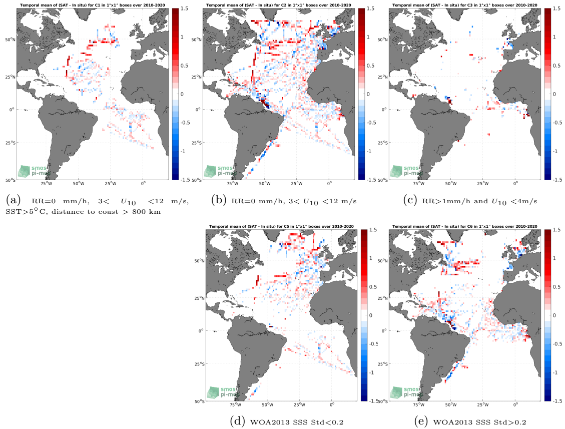
Figure 12: Temporal mean gridded over spatial boxes of size 1^\circ \times 1^\circ of \Delta\text{SSS} (SMOS SSS L3 v335 - 10 Days - 25 km (CATDS-CPDC) - TSG (GOSUD-Research-vessel)) for 5 different subdatasets corresponding to:RR=0 mm/h, 3 < U_{10} < 12 m/s, SST>5°C, distance to coast > 800 km (a), RR=0 mm/h, 3 < U_{10} < 12 m/s (b), RR>1mm/h and U_{10} < 4 m/s (c), WOA2013 SSS Std<0.2 (d), WOA2013 SSS Std>0.2 (e).
