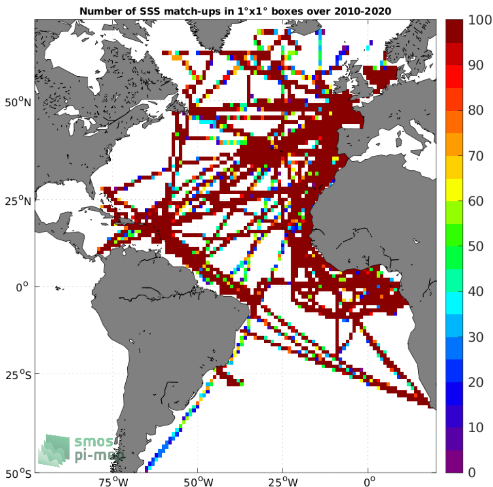
Figure 4: Number of SSS match-ups between TSG (GOSUD-Research-vessel) SSS and the SMOS SSS L3 v335 - 10 Days - 25 km (CATDS-CPDC) SSS product for the Atlantic Ocean Pi-MEP region over 1^\circ \times 1^\circ boxes and for the full satellite product period.
