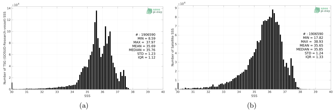
Figure 2: Histograms of SSS from TSG (GOSUD-Research-vessel) (a) and SMOS SSS L3 v335 - 10 Days - 25 km (CATDS-CPDC) (b) considering all match-up pairs per bins of 0.1 over the Atlantic Ocean Pi-MEP region and for the full satellite product period.
