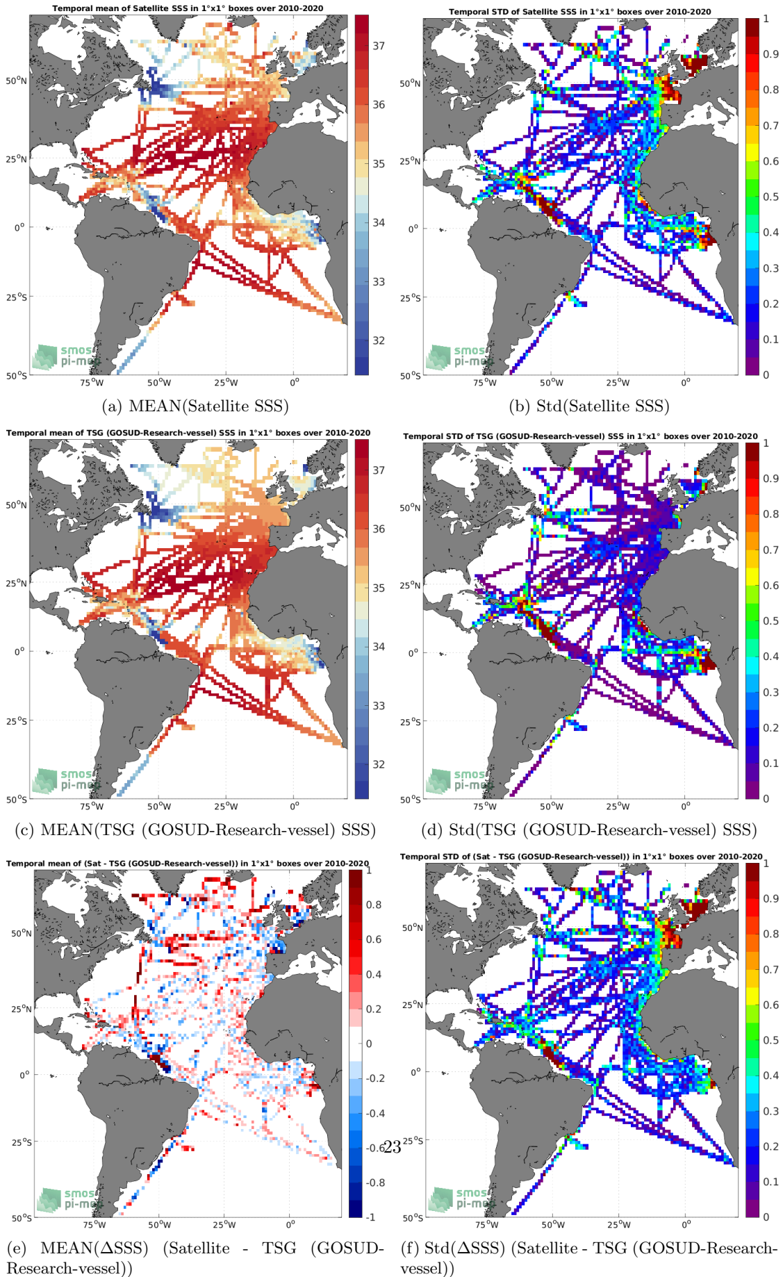
Figure 6: Temporal mean (left) and Std (right) of SSS from SMOS SSS L3 v335 - 10 Days - 25 km (CATDS-CPDC) (top), TSG (GOSUD-Research-vessel) (middle), and of \Delta SSS (Satellite - TSG (GOSUD-Research-vessel)). Only match-up pairs are used to generate these maps.
