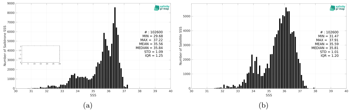
Figure 2: Histograms of SSS from Sairdrone (a) and SMOS SSS L3 v335 - 10 Days - 25 km (CATDS-CPDC) (b) considering all match-up pairs per bins of 0.1 over the Atlantic Ocean Pi-MEP region and for the full satellite product period.
