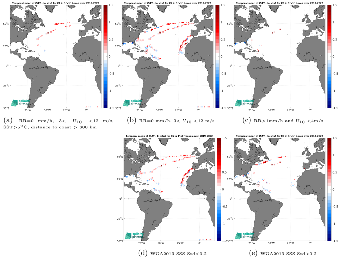
Figure 12: Temporal mean gridded over spatial boxes of size 1^\circ \times 1^\circ of \Delta\text{SSS} (SMOS SSS L3 v335 - 10 Days - 25 km (CATDS-CPDC) - Saildrone) for 5 different subdatasets corresponding to:RR=0 mm/h, 3 < U_{10} < 12 m/s, SST >5^\circ\text{C} , distance to coast > 800 km (a), RR=0 mm/h, 3 < U_{10} < 12 m/s (b), RR >1 mm/h and U_{10} < 4 m/s (c), WOA2013 SSS Std <0.2 (d), WOA2013 SSS Std >0.2 (e).
