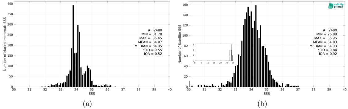
Figure 3: Histograms of SSS from Marine mammals (a) and SMOS SSS L3 v335 - 10 Days - 25 km (CATDS-CPDC) (b) considering all match-up pairs per bins of 0.1 over the Atlantic Ocean Pi-MEP region and for the full satellite product period.
