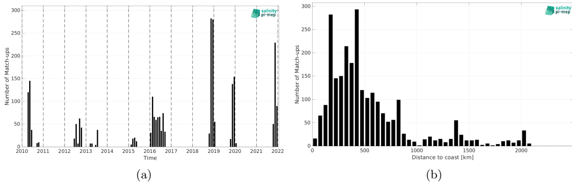
Figure 2: Number of match-ups between Marine mammals and SMOS SSS L3 v335 - 10 Days - 25 km (CATDS-CPDC) SSS as a function of time (a) and as function of the distance to coast (b) over the Atlantic Ocean Pi-MEP region and for the full satellite product period.
