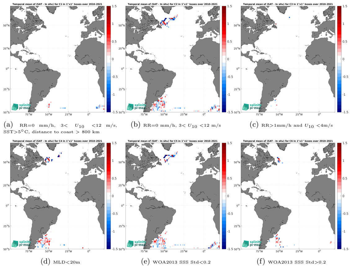
Figure 14: Temporal mean gridded over spatial boxes of size 1^\circ \times 1^\circ of \Delta\text{SSS} (SMOS SSS L3 v335 - 10 Days - 25 km (CATDS-CPDC) - Marine mammals) for 6 different subdatasets corresponding to:RR=0 mm/h, 3 < U_{10} < 12 m/s, SST>5°C, distance to coast > 800 km (a), RR=0 mm/h, 3 < U_{10} < 12 m/s (b), RR>1mm/h and U_{10} < 4 m/s (c),MLD<20m (d),WOA2013 SSS Std<0.2 (e),WOA2013 SSS Std>0.2 (f).
