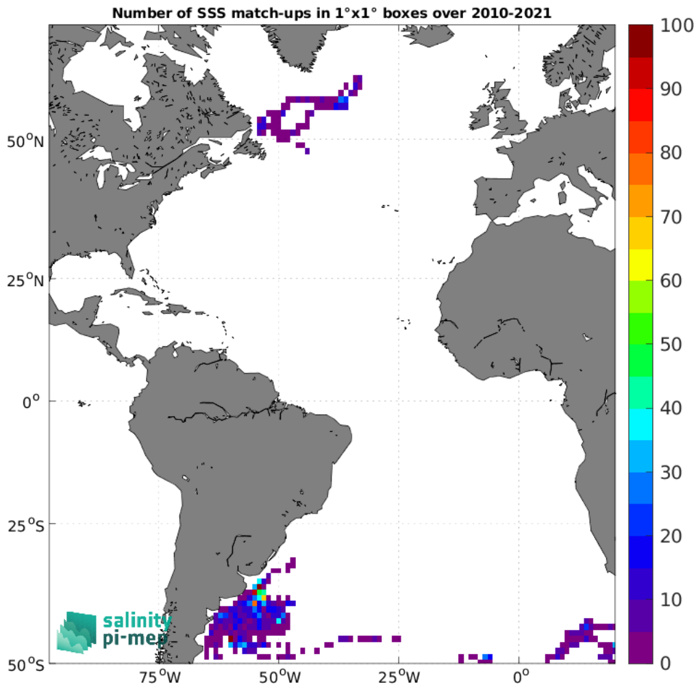
Figure 5: Number of SSS match-ups between Marine mammals SSS and the SMOS SSS L3 v335 - 10 Days - 25 km (CATDS-CPDC) SSS product for the Atlantic Ocean Pi-MEP region over 1^\circ \times 1^\circ boxes and for the full satellite product period.
