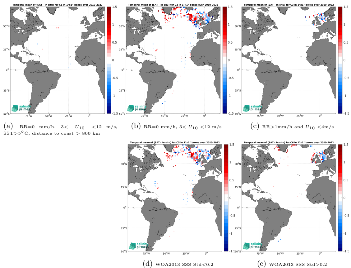
Figure 14: Temporal mean gridded over spatial boxes of size 1^\circ \times 1^\circ of \Delta SSS (SMOS SSS L3 v335 - 10 Days - 25 km (CATDS-CPDC) - ICES) for 5 different subdatasets corresponding to:RR=0 mm/h, 3 < U_{10} < 12 m/s, SST>5°C, distance to coast > 800 km (a), RR=0 mm/h, 3 < U_{10} < 12 m/s (b), RR>1mm/h and U_{10} < 4 m/s (c), WOA2013 SSS Std<0.2 (d), WOA2013 SSS Std>0.2 (e).
