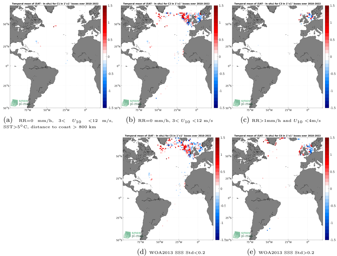
Figure 12: Temporal mean gridded over spatial boxes of size 1^\circ \times 1^\circ of \Delta\text{SSS} (SMOS SSS L3 v335 - 10 Days - 25 km (CATDS-CPDC) - ICES) for 5 different subdatasets corresponding to:RR=0 mm/h, 3 < U_{10} < 12 m/s, SST >5^\circ\text{C} , distance to coast > 800 km (a), RR=0 mm/h, 3 < U_{10} < 12 m/s (b), RR >1 mm/h and U_{10} < 4 m/s (c), WOA2013 SSS Std <0.2 (d), WOA2013 SSS Std >0.2 (e).
