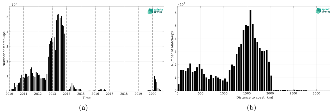
Figure 1: Number of match-ups between Surface drifters and SMOS SSS L3 v335 - 10 Days - 25 km (CATDS-CPDC) SSS as a function of time (a) and as function of the distance to coast (b) over the Atlantic Ocean Pi-MEP region and for the full satellite product period.
