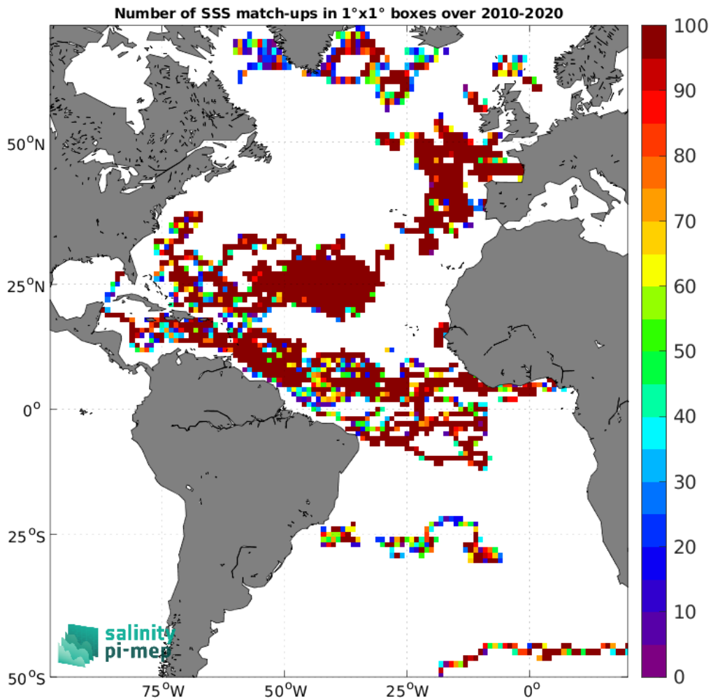
Figure 3: Number of SSS match-ups between Surface drifters SSS and the SMOS SSS L3 v335 - 10 Days - 25 km (CATDS-CPDC) SSS product for the Atlantic Ocean Pi-MEP region over 1°×1° boxes and for the full satellite product period.
