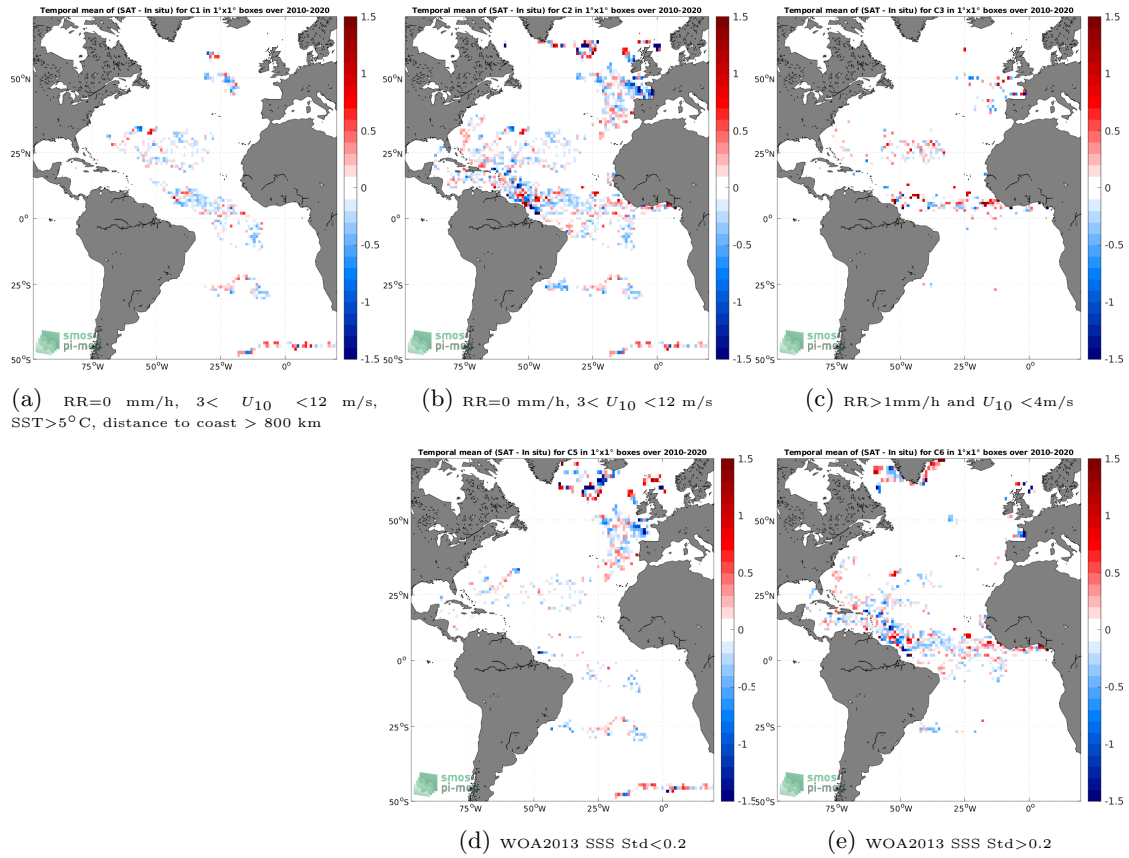
Figure 11: Temporal mean gridded over spatial boxes of size 1^\circ \times 1^\circ of \Delta SSS (SMOS SSS L3 v335 - 10 Days - 25 km (CATDS-CPDC) - Surface drifters) for 5 different subdatasets corresponding to:RR=0 mm/h, 3 < U_{10} < 12 m/s, SST >5^\circ\text{C} , distance to coast > 800 km (a), RR=0 mm/h, 3 < U_{10} < 12 m/s (b), RR >1 mm/h and U_{10} < 4 m/s (c), WOA2013 SSS Std <0.2 (d), WOA2013 SSS Std >0.2 (e).
