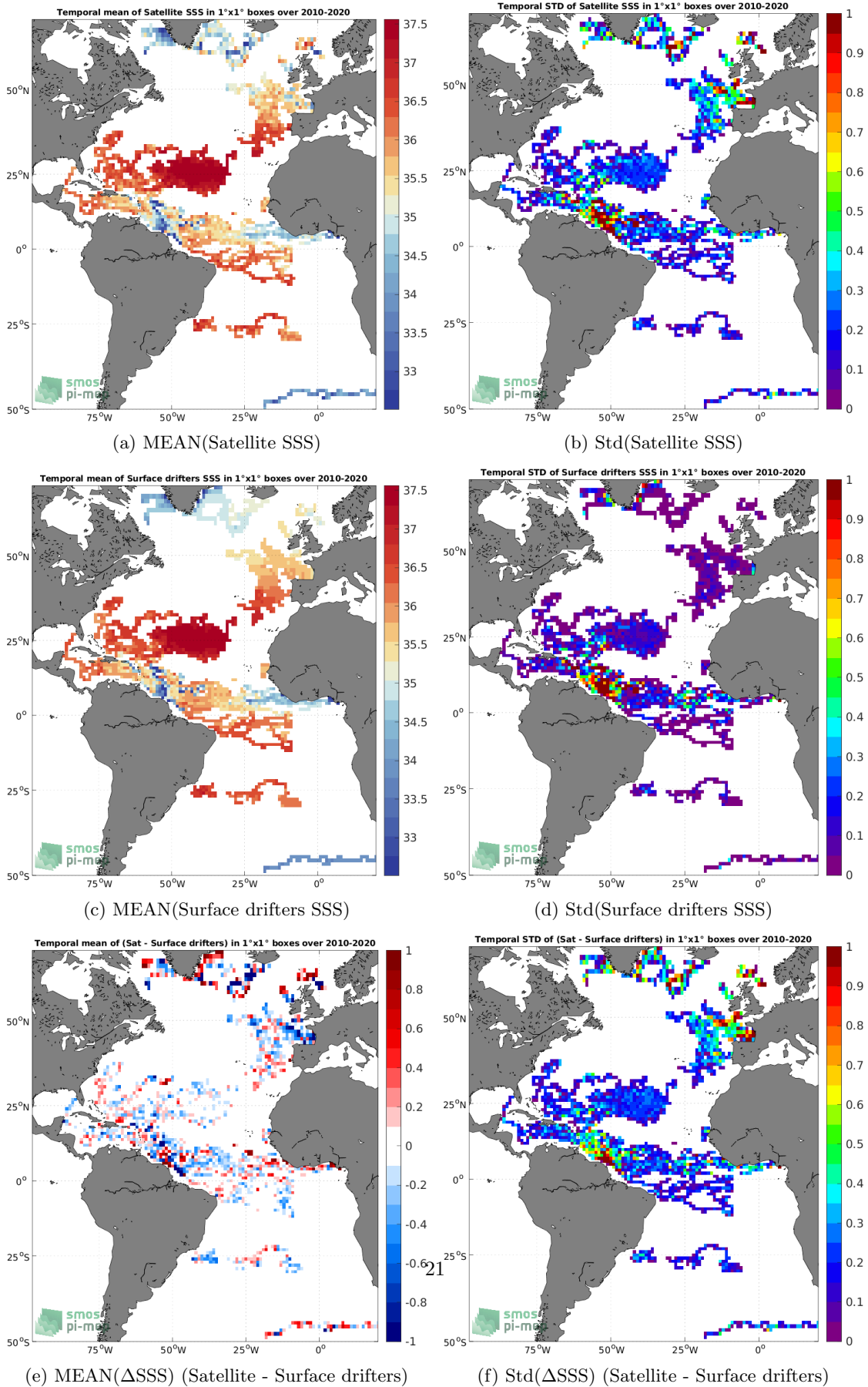
(e) MEAN( \Delta SSS) (Satellite - Surface drifters) (f) Std( \Delta SSS) (Satellite - Surface drifters) Figure 5: Temporal mean (left) and Std (right) of SSS from SMOS SSS L3 v335 - 10 Days - 25 km (CATDS-CPDC) (top), Surface drifters (middle), and of \Delta SSS (Satellite - Surface drifters). Only match-up pairs are used to generate these maps.
