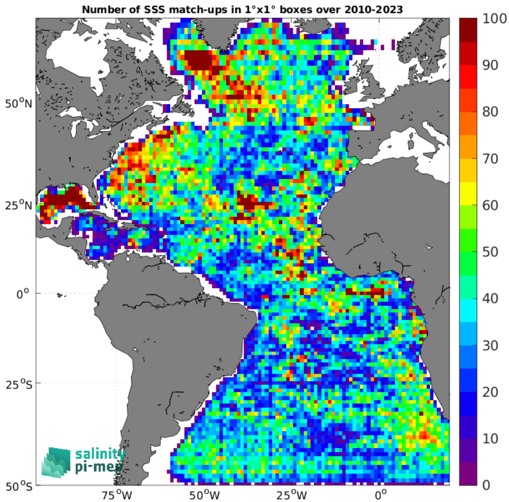
Figure 4: Number of SSS match-ups between Argo SSS and the SMOS SSS L3 v335 - 10 Days - 25 km (CATDS-CPDC) SSS product for the Atlantic Ocean Pi-MEP region over 1^\circ \times 1^\circ boxes and for the full satellite product period.
