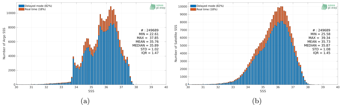
Figure 2: Histograms of SSS from Argo (a) and SMOS SSS L3 v335 - 10 Days - 25 km (CATDS-CPDC) (b) considering all match-up pairs per bins of 0.1 over the Atlantic Ocean Pi-MEP region and for the full satellite product period.
