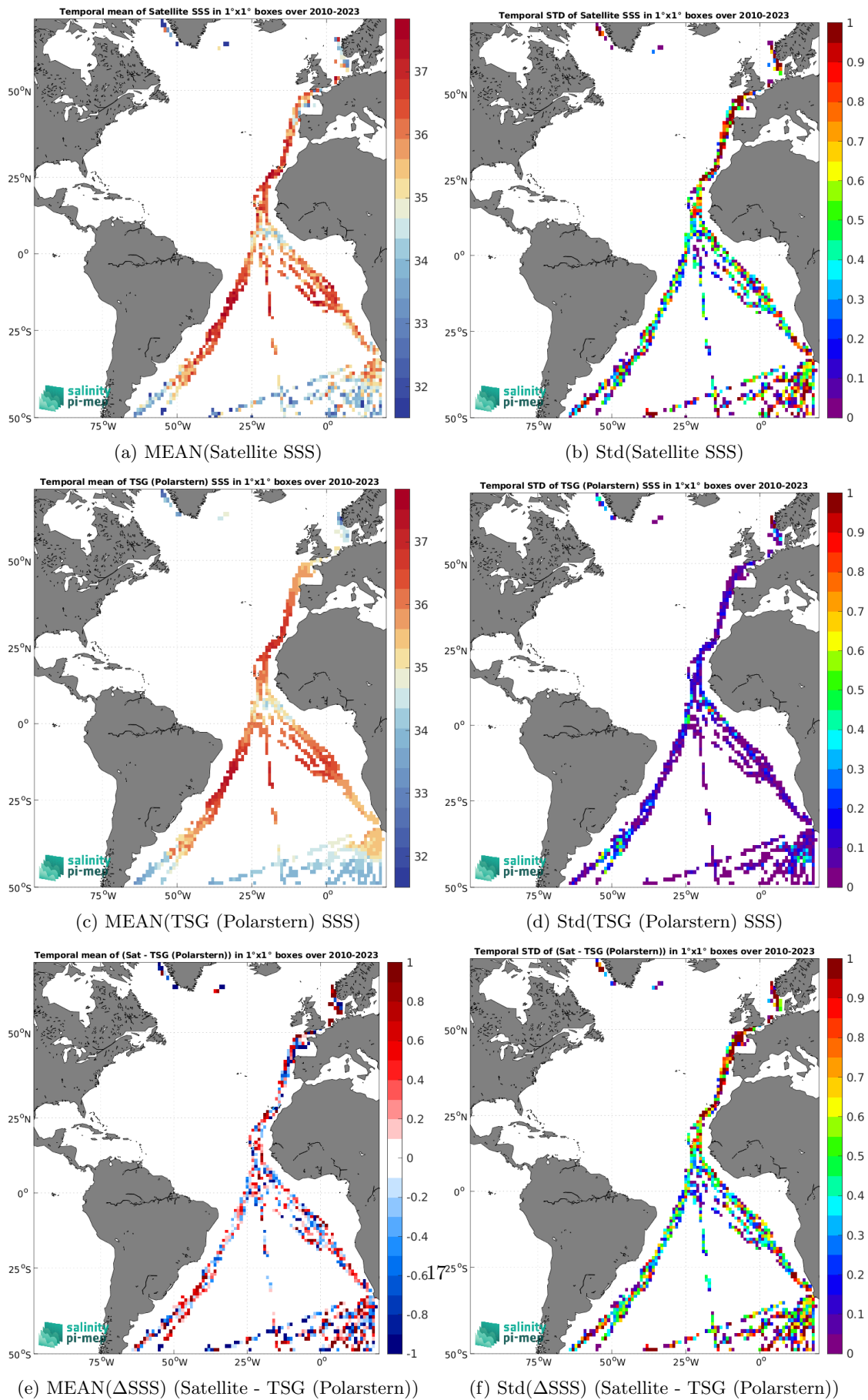
Figure 7: Temporal mean (left) and Std (right) of SSS from SMOS SSS L2Q v333 - 0.25 Deg (CATDS-CPDC) (top), TSG (Polarstern) (middle), and of \Delta SSS (Satellite - TSG (Polarstern)). Only match-up pairs are used to generate these maps.
