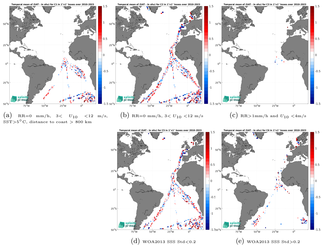
Figure 14: Temporal mean gridded over spatial boxes of size 1^\circ \times 1^\circ of \Delta\text{SSS} (SMOS SSS L2Q v333 - 0.25 Deg (CATDS-CPDC) - TSG (Polarstern)) for 5 different subdatasets corresponding to:RR=0 mm/h, 3 < U_{10} < 12 m/s, SST >5^\circ\text{C} , distance to coast > 800 km (a), RR=0 mm/h, 3 < U_{10} < 12 m/s (b), RR >1 mm/h and U_{10} < 4 m/s (c), WOA2013 SSS Std <0.2 (d), WOA2013 SSS Std >0.2 (e).
