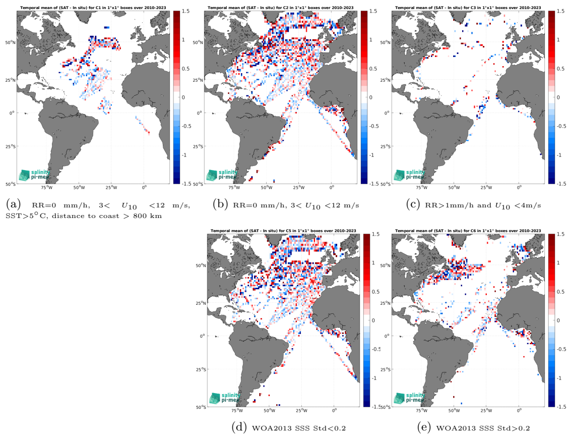
Figure 14: Temporal mean gridded over spatial boxes of size 1^\circ \times 1^\circ of \Delta\text{SSS} (SMOS SSS L2Q v333 - 0.25 Deg (CATDS-CPDC) - TSG (LEGOS-DM)) for 5 different subdatasets corresponding to:RR=0 mm/h, 3 < U_{10} < 12 m/s, SST >5^\circ\text{C} , distance to coast > 800 km (a), RR=0 mm/h, 3 < U_{10} < 12 m/s (b), RR >1 mm/h and U_{10} < 4 m/s (c), WOA2013 SSS Std <0.2 (d), WOA2013 SSS Std >0.2 (e).
