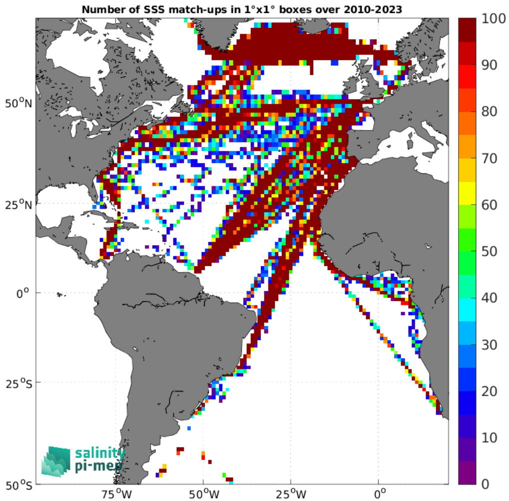
Figure 5: Number of SSS match-ups between TSG (LEGOS-DM) SSS and the SMOS SSS L2Q v333 - 0.25 Deg (CATDS-CPDC) SSS product for the Atlantic Ocean Pi-MEP region over 1^\circ \times 1^\circ boxes and for the full satellite product period.
