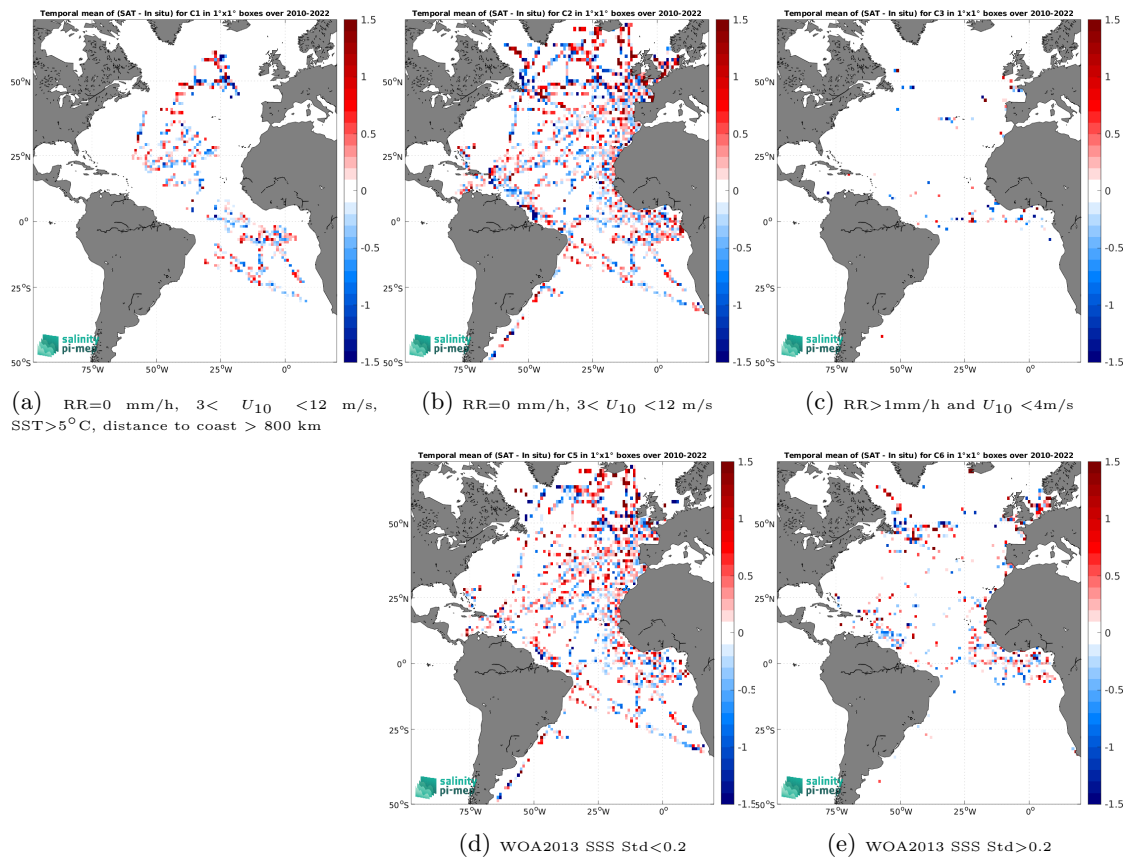
Figure 14: Temporal mean gridded over spatial boxes of size 1^\circ \times 1^\circ of \Delta\text{SSS} (SMOS SSS L2Q v333 - 0.25 Deg (CATDS-CPDC) - TSG (GOSUD-Research-vessel)) for 5 different subdatasets corresponding to:RR=0 mm/h, 3 < U_{10} < 12 m/s, SST >5^\circ\text{C} , distance to coast > 800 km (a), RR=0 mm/h, 3 < U_{10} < 12 m/s (b), RR >1 mm/h and U_{10} < 4 m/s (c), WOA2013 SSS Std <0.2 (d), WOA2013 SSS Std >0.2 (e).
