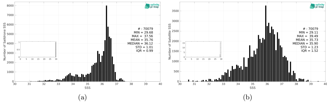
Figure 3: Histograms of SSS from Saildrone (a) and SMOS SSS L2Q v333 - 0.25 Deg (CATDS-CPDC) (b) considering all match-up pairs per bins of 0.1 over the Atlantic Ocean Pi-MEP region and for the full satellite product period.
