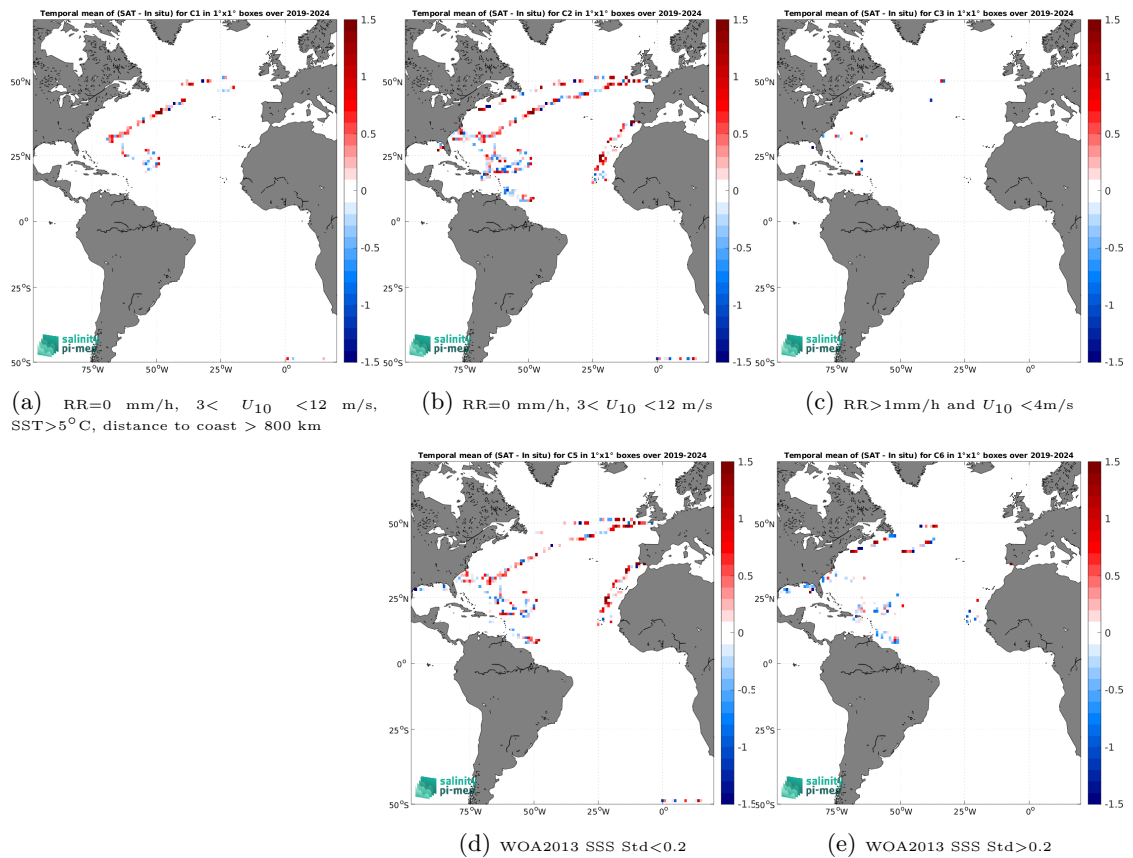
Figure 14: Temporal mean gridded over spatial boxes of size 1^\circ \times 1^\circ of \Delta\text{SSS} (SMOS SSS L2Q v333 - 0.25 Deg (CATDS-CPDC) - Sailydrone) for 5 different subdatasets corresponding to:RR=0 mm/h, 3 < U_{10} < 12 m/s, SST >5^\circ\text{C} , distance to coast > 800 km (a), RR=0 mm/h, 3 < U_{10} < 12 m/s (b), RR >1 mm/h and U_{10} < 4 m/s (c), WOA2013 SSS Std <0.2 (d), WOA2013 SSS Std >0.2 (e).
