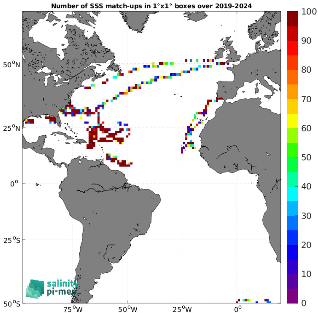
Figure 5: Number of SSS match-ups between Saildrone SSS and the SMOS SSS L2Q v333 - 0.25 Deg (CATDS-CPDC) SSS product for the Atlantic Ocean Pi-MEP region over 1°x1° boxes and for the full satellite product period.
