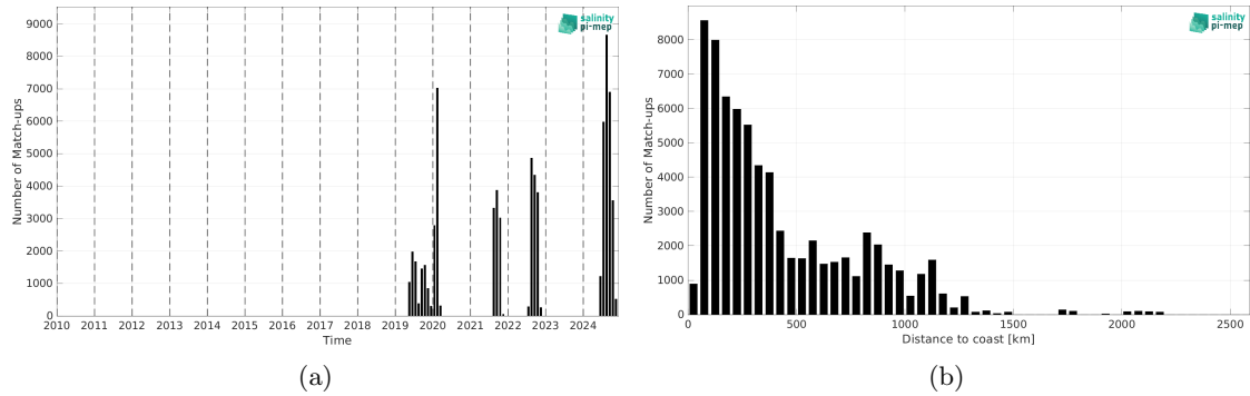
Figure 2: Number of match-ups between Saildrone and SMOS SSS L2Q v333 - 0.25 Deg (CATDS-CPDC) SSS as a function of time (a) and as function of the distance to coast (b) over the Atlantic Ocean Pi-MEP region and for the full satellite product period.
