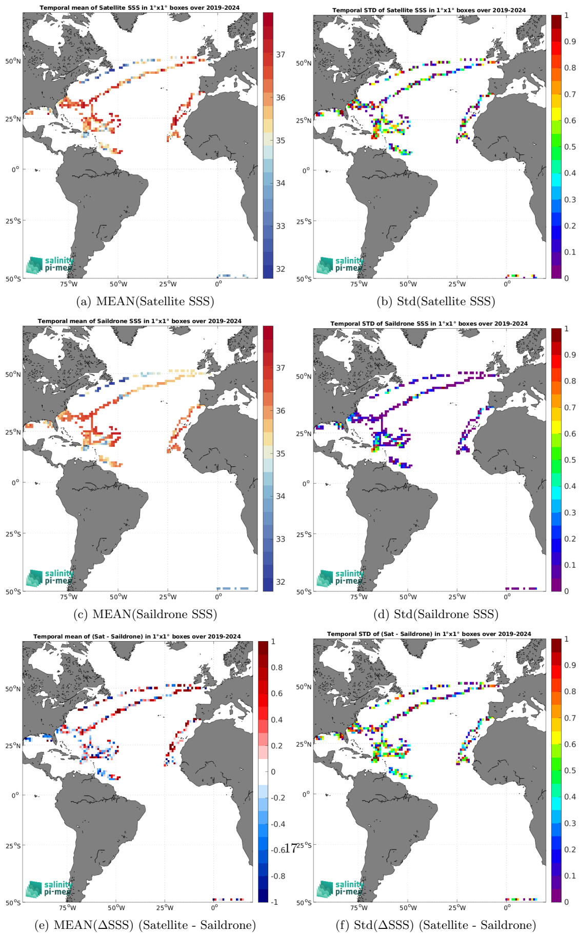
Figure 7: Temporal mean (left) and Std (right) of SSS from SMOS SSS L2Q v333 - 0.25 Deg (CATDS-CPDC) (top), Saildrone (middle), and of \Delta SSS (Satellite - Saildrone). Only match-up pairs are used to generate these maps.
