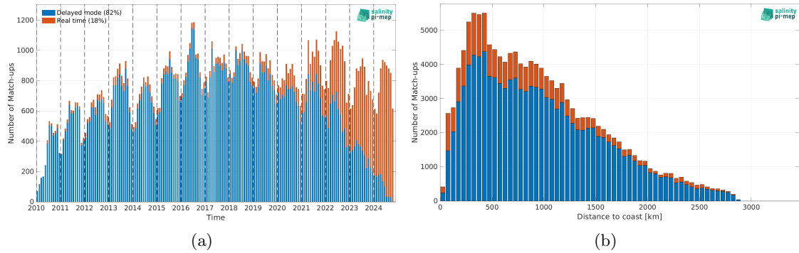
Figure 2: Number of match-ups between Argo and SMOS SSS L2Q v333 - 0.25 Deg (CATDS-CPDC) SSS as a function of time (a) and as function of the distance to coast (b) over the Atlantic Ocean Pi-MEP region and for the full satellite product period.
