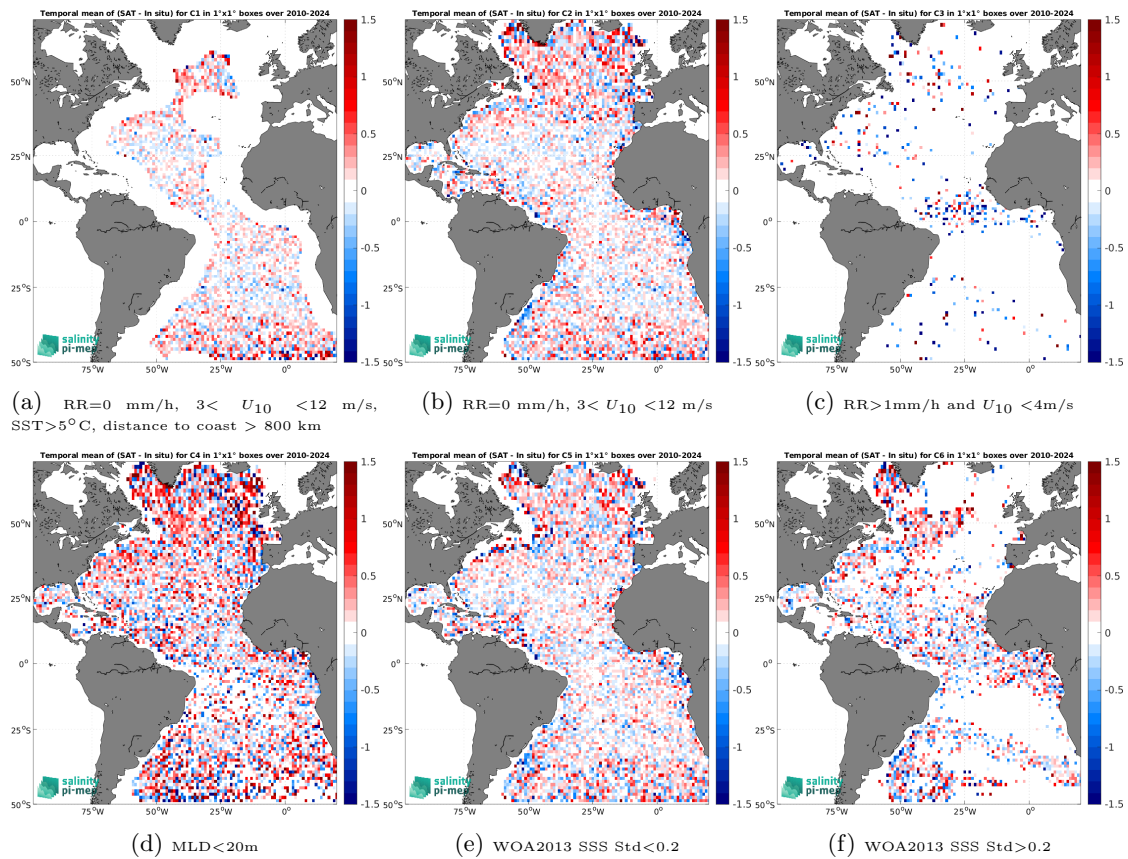
Figure 14: Temporal mean gridded over spatial boxes of size 1^\circ \times 1^\circ of \Delta SSS (SMOS SSS L2Q v333 - 0.25 Deg (CATDS-CPDC) - Argo) for 6 different subdatasets corresponding to:RR=0 mm/h, 3 < U_{10} < 12 m/s, SST>5°C, distance to coast > 800 km (a), RR=0 mm/h, 3 < U_{10} < 12 m/s (b), RR>1mm/h and U_{10} < 4 m/s (c),MLD<20m (d),WOA2013 SSS Std<0.2 (e),WOA2013 SSS Std>0.2 (f).
