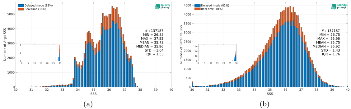
Figure 3: Histograms of SSS from Argo (a) and SMOS SSS L2Q v333 - 0.25 Deg (CATDS-CPDC) (b) considering all match-up pairs per bins of 0.1 over the Atlantic Ocean Pi-MEP region and for the full satellite product period.
