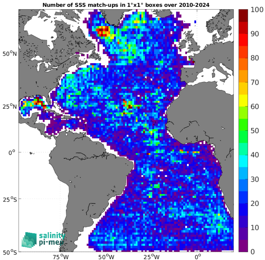
Figure 5: Number of SSS match-ups between Argo SSS and the SMOS SSS L2Q v333 - 0.25 Deg (CATDS-CPDC) SSS product for the Atlantic Ocean Pi-MEP region over 1^\circ \times 1^\circ boxes and for the full satellite product period.
