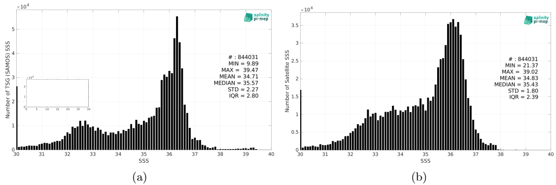
Figure 2: Histograms of SSS from TSG (SAMOS) (a) and SMOS SSS L3 v332 - 9 Days (CATDS-CPDC) (b) considering all match-up pairs per bins of 0.1 over the Atlantic Ocean Pi-MEP region and for the full satellite product period.
