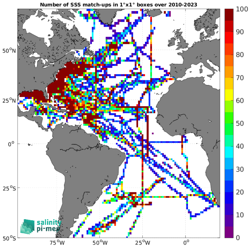
Figure 4: Number of SSS match-ups between TSG (SAMOS) SSS and the SMOS SSS L3 v332 - 9 Days (CATDS-CPDC) SSS product for the Atlantic Ocean Pi-MEP region over 1^\circ \times 1^\circ boxes and for the full satellite product period.
