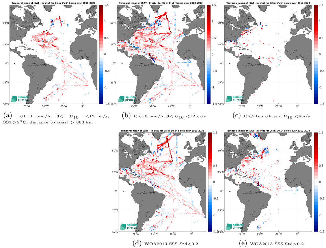
Figure 12: Temporal mean gridded over spatial boxes of size 1^\circ \times 1^\circ of \Delta SSS (SMOS SSS L3 v332 - 9 Days (CATDS-CPDC) - TSG (SAMOS)) for 5 different subdatasets corresponding to:RR=0 mm/h, 3 < U_{10} < 12 m/s, SST >5^\circ\text{C} , distance to coast > 800 km (a), RR=0 mm/h, 3 < U_{10} < 12 m/s (b), RR >1 mm/h and U_{10} < 4 m/s (c), WOA2013 SSS Std <0.2 (d), WOA2013 SSS Std >0.2 (e).
