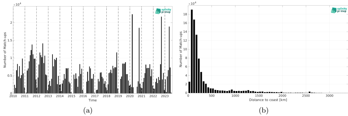
Figure 1: Number of match-ups between TSG (SAMOS) and SMOS SSS L3 v332 - 9 Days (CATDS-CPDC) SSS as a function of time (a) and as function of the distance to coast (b) over the Atlantic Ocean Pi-MEP region and for the full satellite product period.
