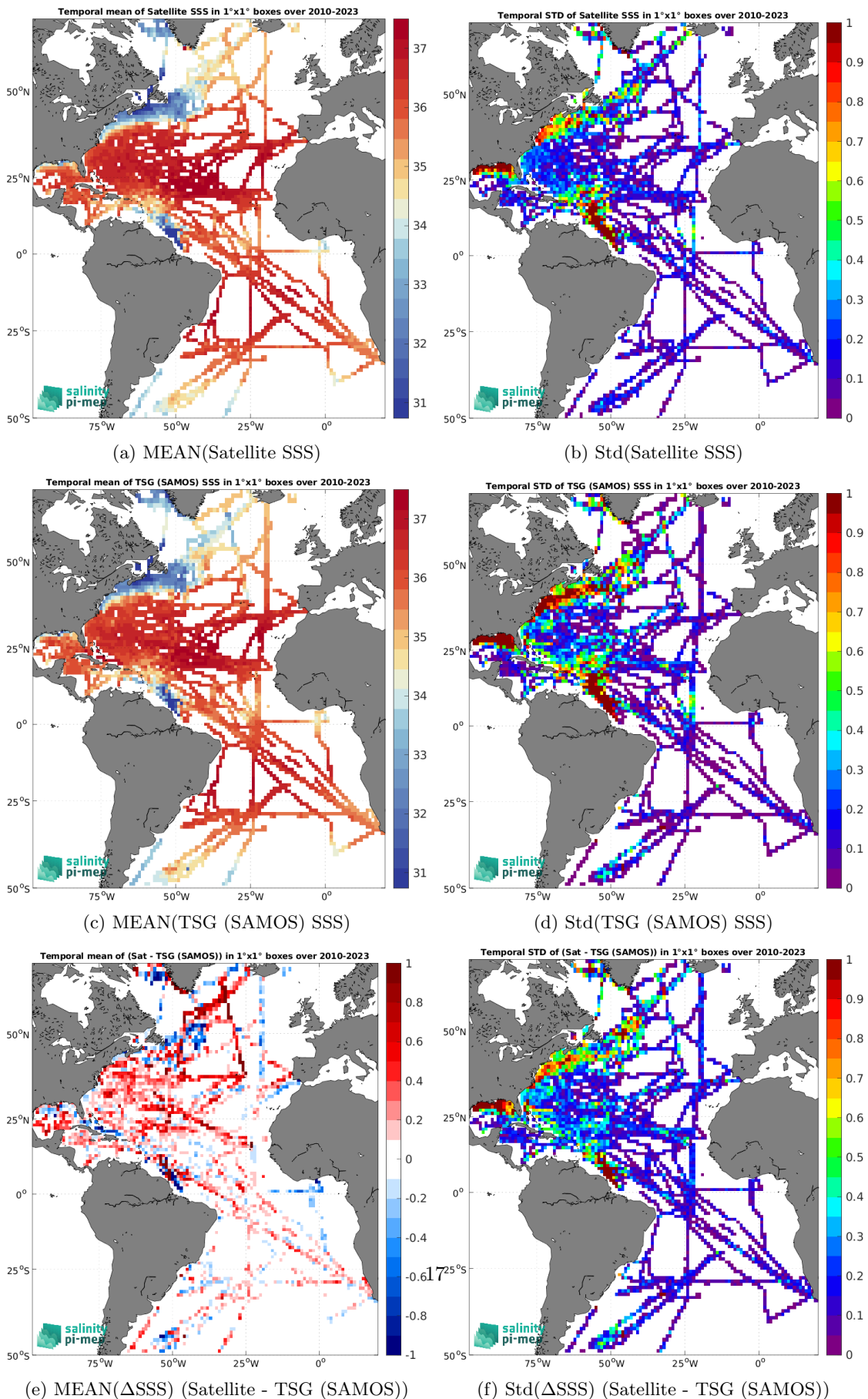
Figure 6: Temporal mean (left) and Std (right) of SSS from SMOS SSS L3 v332 - 9 Days (CATDS-CPDC) (top), TSG (SAMOS) (middle), and of \Delta SSS (Satellite - TSG (SAMOS)). Only match-up pairs are used to generate these maps.
