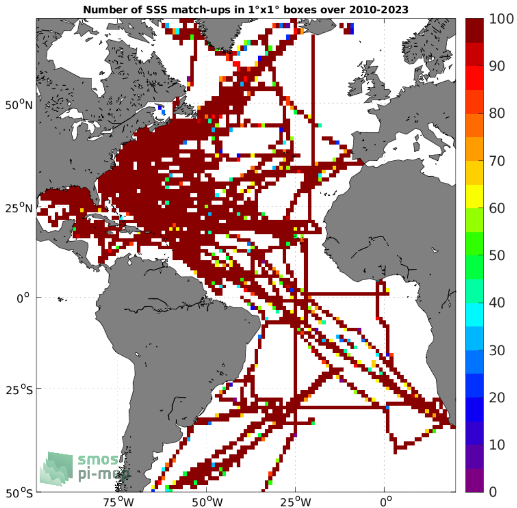
Figure 4: Number of SSS match-ups between TSG (SAMOS) SSS and the SMOS SSS L3 v332 - 9 Days (CATDS-CPDC) SSS product for the Atlantic Ocean Pi-MEP region over 1°x1° boxes and for the full satellite product period.
