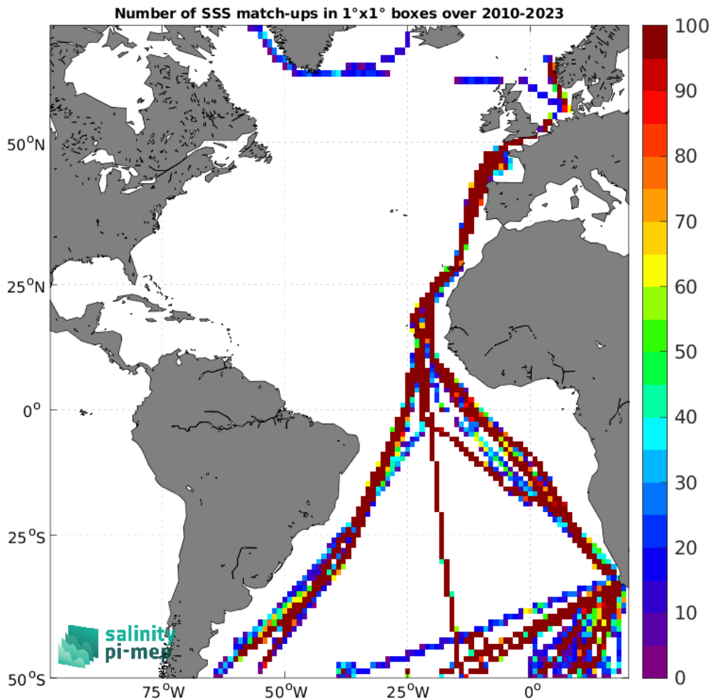
Figure 5: Number of SSS match-ups between TSG (Polarstern) SSS and the SMOS SSS L3 v332 - 9 Days (CATDS-CPDC) SSS product for the Atlantic Ocean Pi-MEP region over 1^\circ \times 1^\circ boxes and for the full satellite product period.
