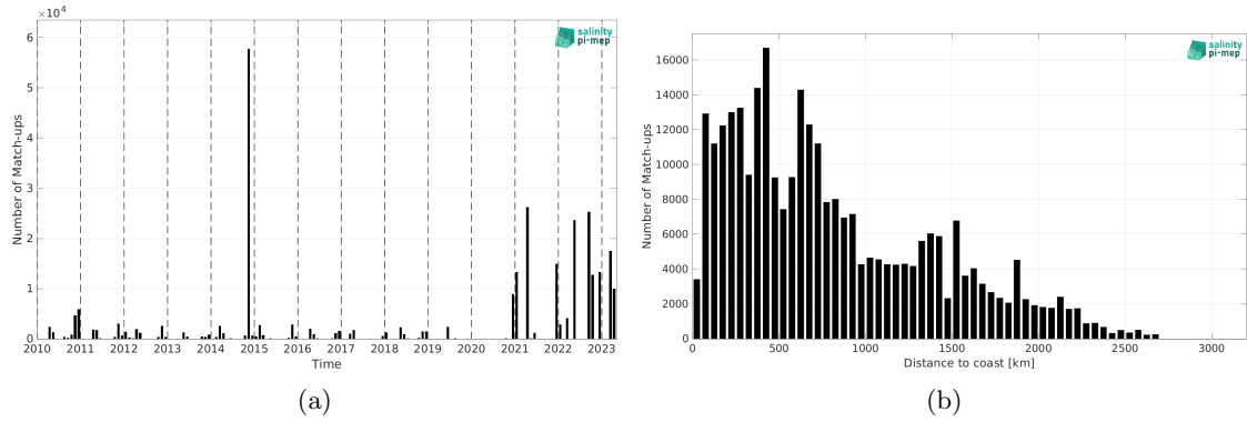
Figure 2: Number of match-ups between TSG (Polarstern) and SMOS SSS L3 v332 - 9 Days (CATDS-CPDC) SSS as a function of time (a) and as function of the distance to coast (b) over the Atlantic Ocean Pi-MEP region and for the full satellite product period.
