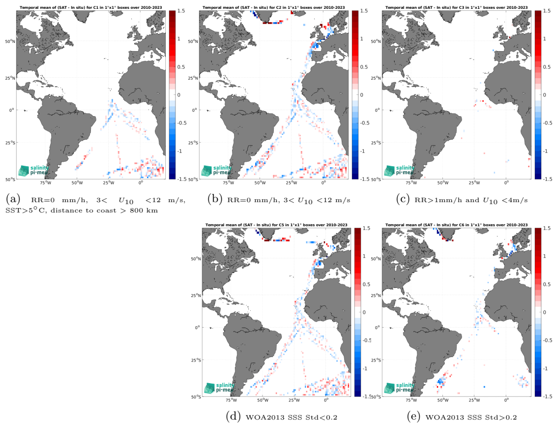
Figure 14: Temporal mean gridded over spatial boxes of size 1^\circ \times 1^\circ of \Delta\text{SSS} (SMOS SSS L3 v332 - 9 Days (CATDS-CPDC) - TSG (Polarstern)) for 5 different subdatasets corresponding to:RR=0 mm/h, 3 < U_{10} < 12 m/s, SST >5^\circ\text{C} , distance to coast > 800 km (a), RR=0 mm/h, 3 < U_{10} < 12 m/s (b), RR >1 mm/h and U_{10} < 4 m/s (c), WOA2013 SSS Std <0.2 (d), WOA2013 SSS Std >0.2 (e).
