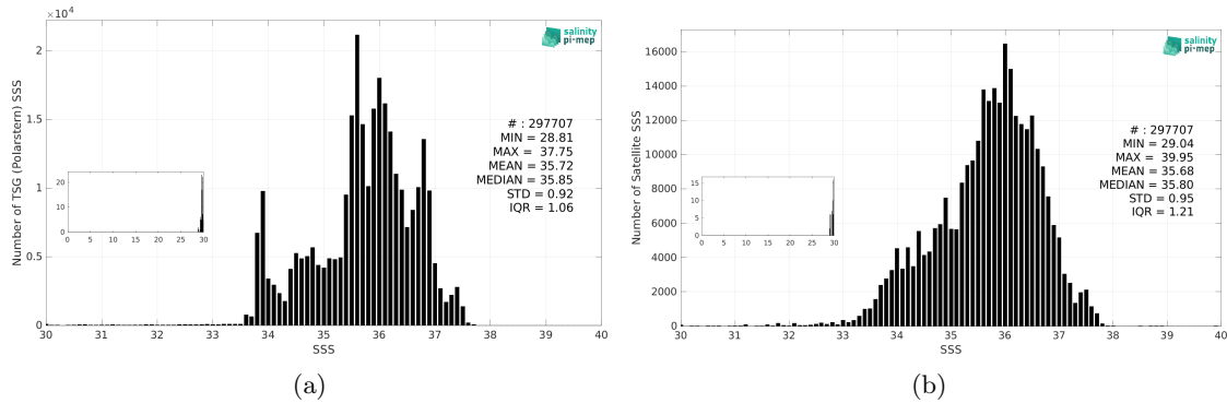
Figure 3: Histograms of SSS from TSG (Polarstern) (a) and SMOS SSS L3 v332 - 9 Days (CATDS-CPDC) (b) considering all match-up pairs per bins of 0.1 over the Atlantic Ocean Pi-MEP region and for the full satellite product period.
