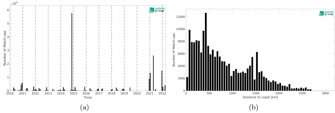
Figure 1: Number of match-ups between TSG (Polarstern) and SMOS SSS L3 v332 - 9 Days (CATDS-CPDC) SSS as a function of time (a) and as function of the distance to coast (b) over the Atlantic Ocean Pi-MEP region and for the full satellite product period.
