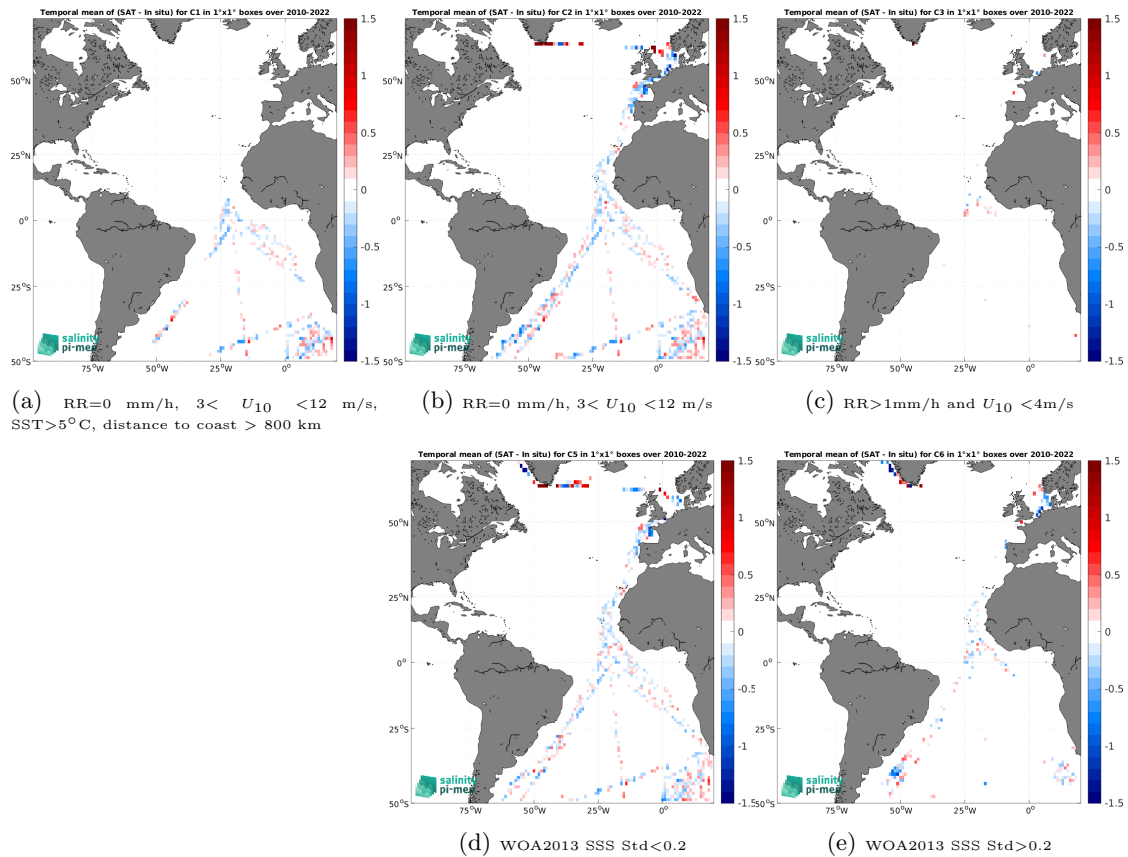
Figure 12: Temporal mean gridded over spatial boxes of size 1^\circ \times 1^\circ of \Delta\text{SSS} (SMOS SSS L3 v332 - 9 Days (CATDS-CPDC) - TSG (Polarstern)) for 5 different subdatasets corresponding to:RR=0 mm/h, 3 < U_{10} < 12 m/s, SST >5^\circ\text{C} , distance to coast > 800 km (a), RR=0 mm/h, 3 < U_{10} < 12 m/s (b), RR >1 mm/h and U_{10} < 4 m/s (c), WOA2013 SSS Std <0.2 (d), WOA2013 SSS Std >0.2 (e).
