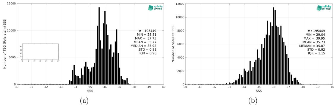
Figure 2: Histograms of SSS from TSG (Polarstern) (a) and SMOS SSS L3 v332 - 9 Days (CATDS-CPDC) (b) considering all match-up pairs per bins of 0.1 over the Atlantic Ocean Pi-MEP region and for the full satellite product period.
