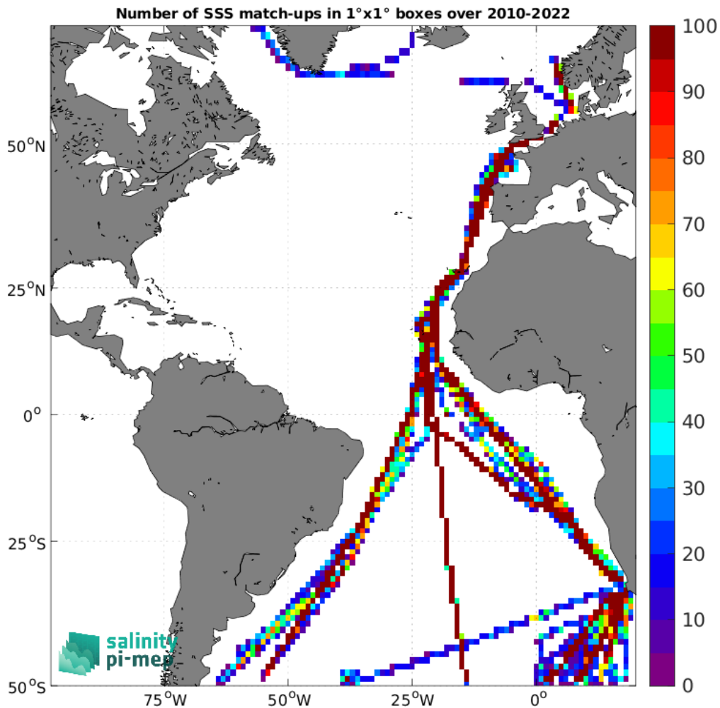
Figure 4: Number of SSS match-ups between TSG (Polarstern) SSS and the SMOS SSS L3 v332 - 9 Days (CATDS-CPDC) SSS product for the Atlantic Ocean Pi-MEP region over 1^\circ \times 1^\circ boxes and for the full satellite product period.
