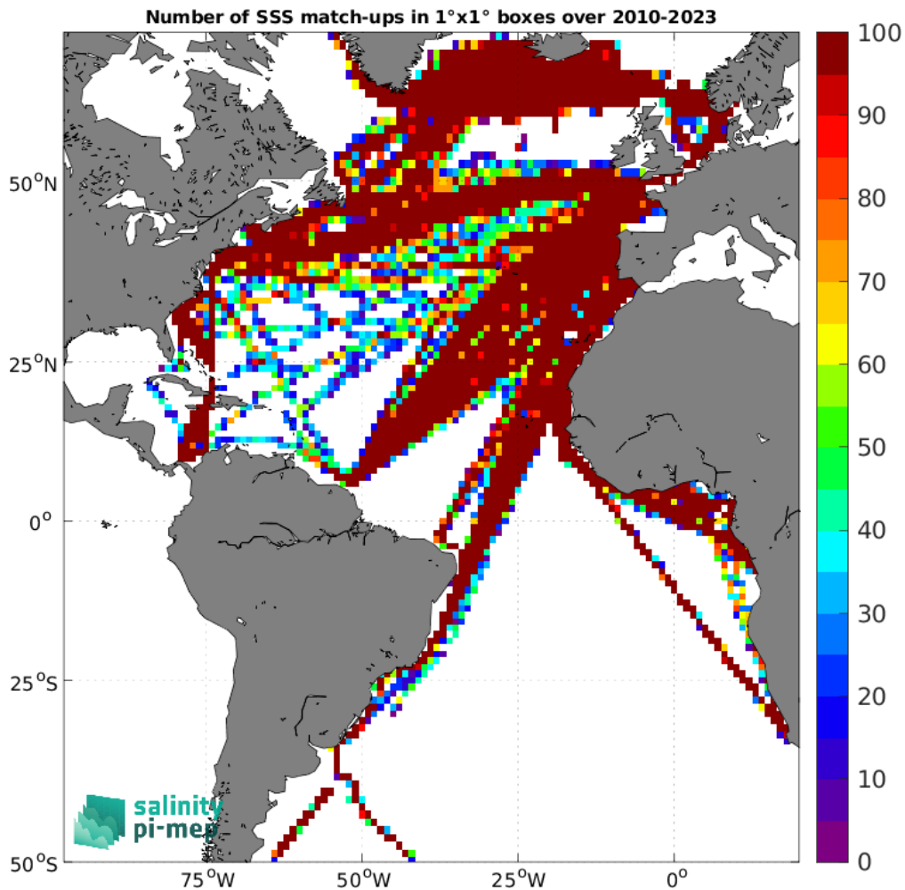
Figure 5: Number of SSS match-ups between TSG (LEGOS-DM) SSS and the SMOS SSS L3 v332 - 9 Days (CATDS-CPDC) SSS product for the Atlantic Ocean Pi-MEP region over 1°x1° boxes and for the full satellite product period.
