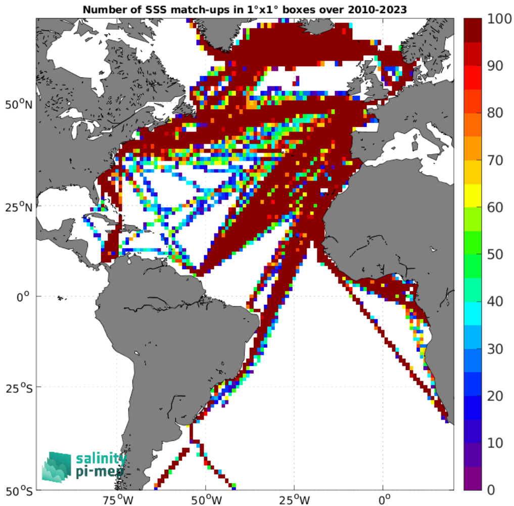
Figure 4: Number of SSS match-ups between TSG (LEGOS-DM) SSS and the SMOS SSS L3 v332 - 9 Days (CATDS-CPDC) SSS product for the Atlantic Ocean Pi-MEP region over 1^\circ \times 1^\circ boxes and for the full satellite product period.
