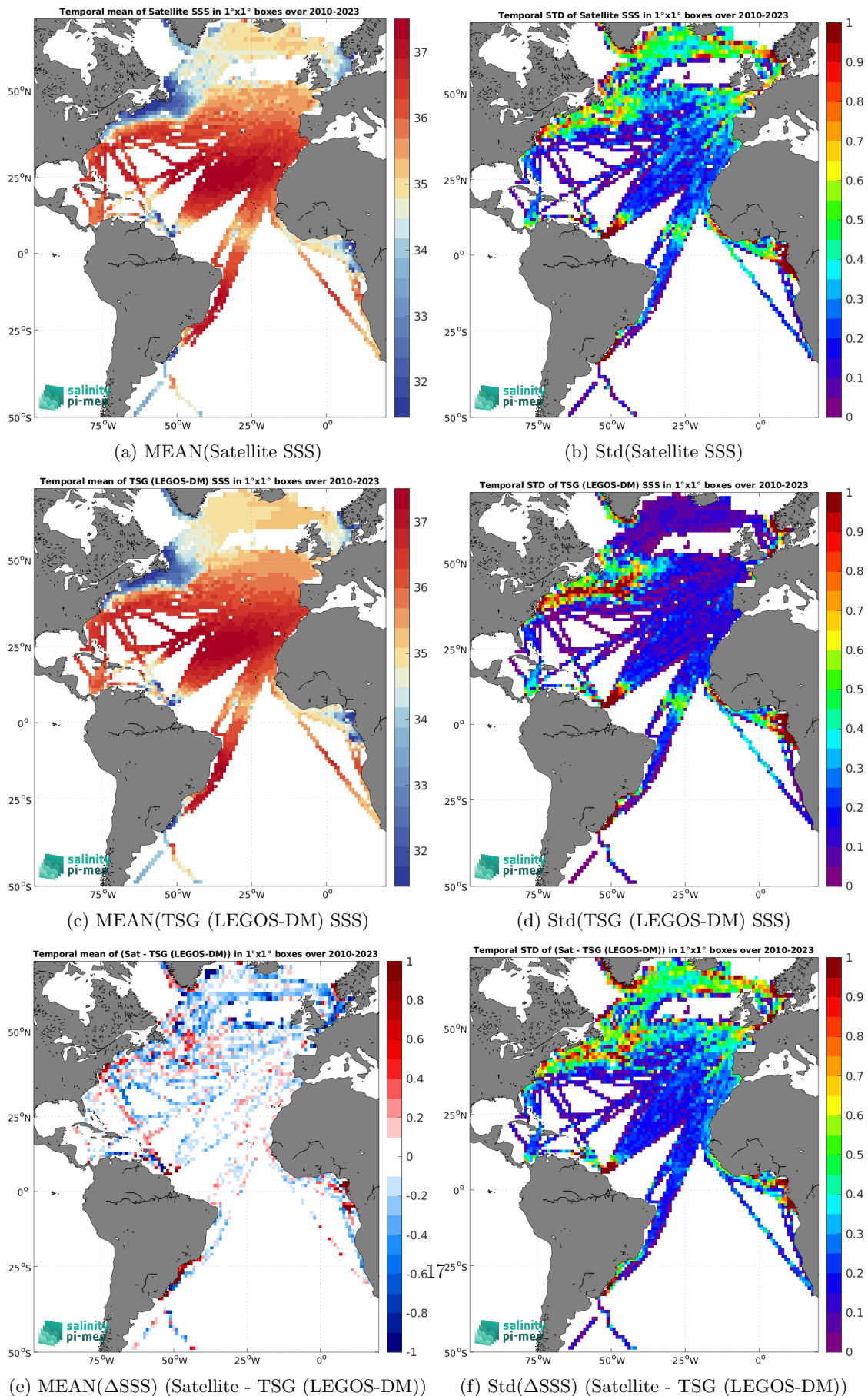
Figure 6: Temporal mean (left) and Std (right) of SSS from SMOS SSS L3 v332 - 9 Days (CATDS-CPDC) (top), TSG (LEGOS-DM) (middle), and of \Delta SSS (Satellite - TSG (LEGOS-DM)). Only match-up pairs are used to generate these maps.
