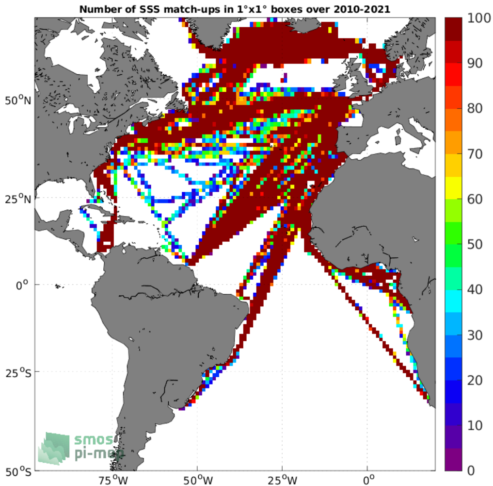
Figure 4: Number of SSS match-ups between TSG (LEGOS-DM) SSS and the SMOS SSS L3 v332 - 9 Days (CATDS-CPDC) SSS product for the Atlantic Ocean Pi-MEP region over 1°x1° boxes and for the full satellite product period.
