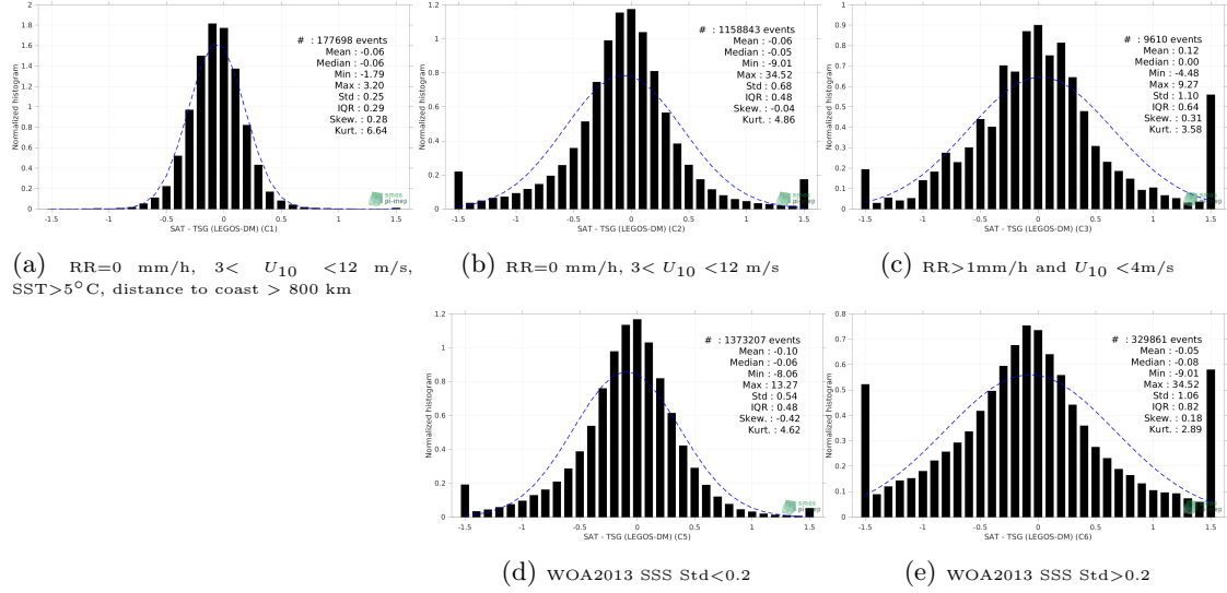
Figure 13: Normalized histogram of \Delta SSS (SMOS SSS L3 v332 - 9 Days (CATDS-CPDC) - TSG (LEGOS-DM)) for 5 different subdatasets corresponding to: RR=0 mm/h, 3 < U_{10} < 12 m/s, SST>5°C, distance to coast > 800 km (a), RR=0 mm/h, 3 < U_{10} < 12 m/s (b), RR>1mm/h and U_{10} < 4 m/s (c), WOA2013 SSS Std<0.2 (d), WOA2013 SSS Std>0.2 (e).
