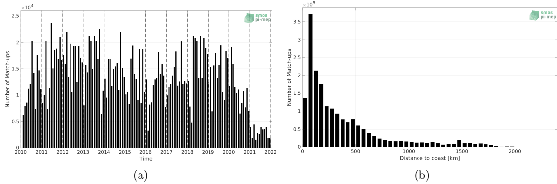
Figure 1: Number of match-ups between TSG (LEGOS-DM) and SMOS SSS L3 v332 - 9 Days (CATDS-CPDC) SSS as a function of time (a) and as function of the distance to coast (b) over the Atlantic Ocean Pi-MEP region and for the full satellite product period.
