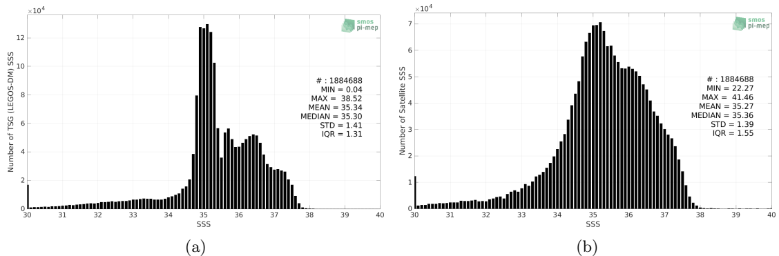
Figure 2: Histograms of SSS from TSG (LEGOS-DM) (a) and SMOS SSS L3 v332 - 9 Days (CATDS-CPDC) (b) considering all match-up pairs per bins of 0.1 over the Atlantic Ocean Pi-MEP region and for the full satellite product period.
