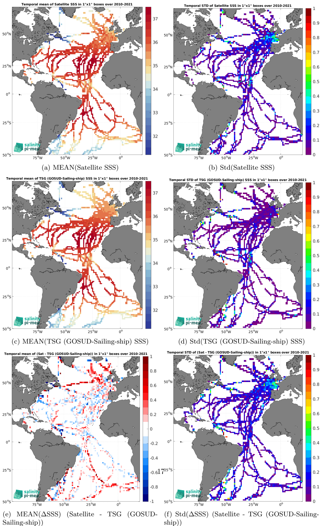
Figure 7: Temporal mean (left) and Std (right) of SSS from SMOS SSS L3 v332 - 9 Days (CATDS-CPDC) (top), TSG (GOSUD-Sailing-ship) (middle), and of \Delta SSS (Satellite - TSG (GOSUD-Sailing-ship)). Only match-up pairs are used to generate these maps.
