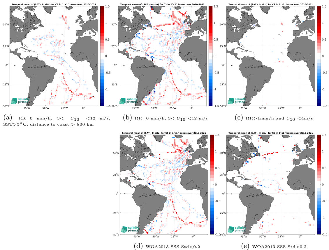
Figure 14: Temporal mean gridded over spatial boxes of size 1^\circ \times 1^\circ of \Delta SSS (SMOS SSS L3 v332 - 9 Days (CATDS-CPDC) - TSG (GOSUD-Sailing-ship)) for 5 different subdatasets corresponding to:RR=0 mm/h, 3 < U_{10} < 12 m/s, SST >5^\circ\text{C} , distance to coast > 800 km (a), RR=0 mm/h, 3 < U_{10} < 12 m/s (b), RR >1 mm/h and U_{10} < 4 m/s (c), WOA2013 SSS Std <0.2 (d), WOA2013 SSS Std >0.2 (e).
