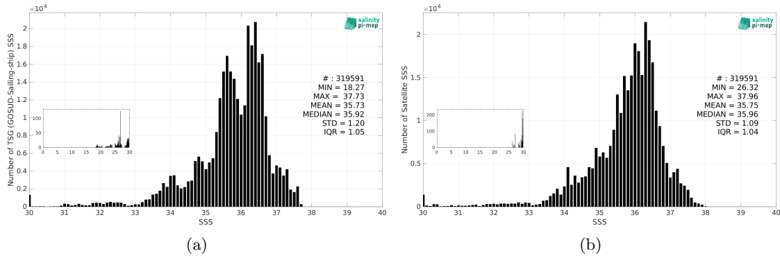
Figure 3: Histograms of SSS from TSG (GOSUD-Sailing-ship) (a) and SMOS SSS L3 v332 - 9 Days (CATDS-CPDC) (b) considering all match-up pairs per bins of 0.1 over the Atlantic Ocean Pi-MEP region and for the full satellite product period.
