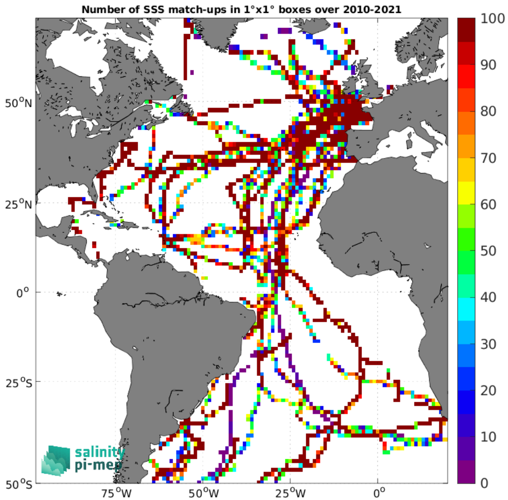
Figure 5: Number of SSS match-ups between TSG (GOSUD-Sailing-ship) SSS and the SMOS SSS L3 v332 - 9 Days (CATDS-CPDC) SSS product for the Atlantic Ocean Pi-MEP region over 1^\circ \times 1^\circ boxes and for the full satellite product period.
