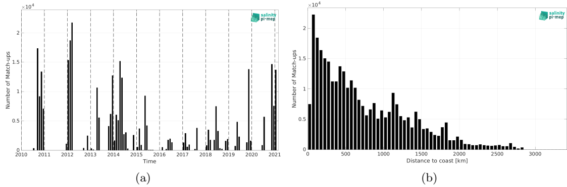
Figure 2: Number of match-ups between TSG (GOSUD-Sailing-ship) and SMOS SSS L3 v332 - 9 Days (CATDS-CPDC) SSS as a function of time (a) and as function of the distance to coast (b) over the Atlantic Ocean Pi-MEP region and for the full satellite product period.
