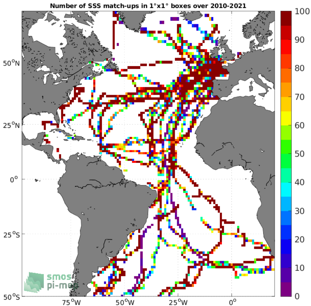
Figure 4: Number of SSS match-ups between TSG (GOSUD-Sailing-ship) SSS and the SMOS SSS L3 v332 - 9 Days (CATDS-CPDC) SSS product for the Atlantic Ocean Pi-MEP region over 1°x1° boxes and for the full satellite product period.
