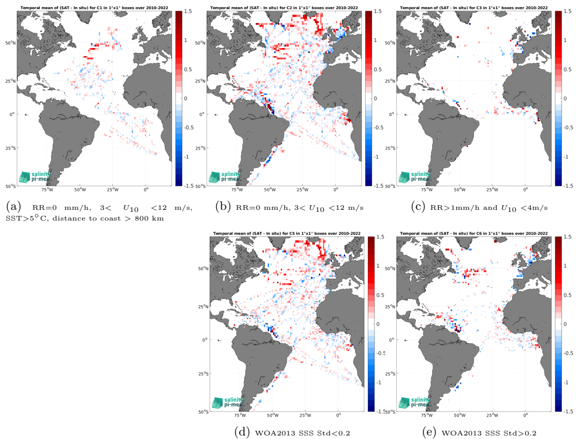
Figure 14: Temporal mean gridded over spatial boxes of size 1^\circ \times 1^\circ of \Delta\text{SSS} (SMOS SSS L3 v332 - 9 Days (CATDS-CPDC) - TSG (GOSUD-Research-vessel)) for 5 different subdatasets corresponding to:RR=0 mm/h, 3 < U_{10} < 12 m/s, SST>5°C, distance to coast > 800 km (a), RR=0 mm/h, 3 < U_{10} < 12 m/s (b), RR>1mm/h and U_{10} < 4 m/s (c), WOA2013 SSS Std<0.2 (d), WOA2013 SSS Std>0.2 (e).
