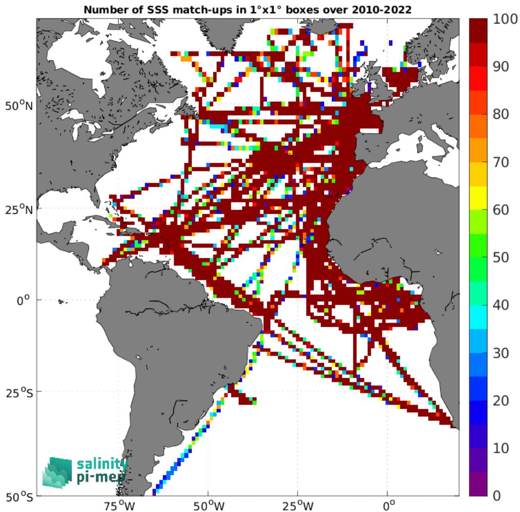
Figure 5: Number of SSS match-ups between TSG (GOSUD-Research-vessel) SSS and the SMOS SSS L3 v332 - 9 Days (CATDS-CPDC) SSS product for the Atlantic Ocean Pi-MEP region over 1° × 1° boxes and for the full satellite product period.
