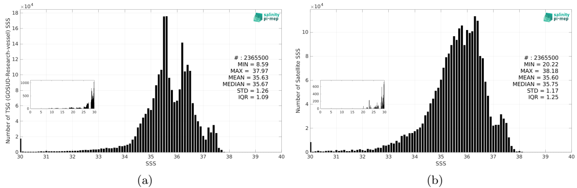
Figure 3: Histograms of SSS from TSG (GOSUD-Research-vessel) (a) and SMOS SSS L3 v332 - 9 Days (CATDS-CPDC) (b) considering all match-up pairs per bins of 0.1 over the Atlantic Ocean Pi-MEP region and for the full satellite product period.
