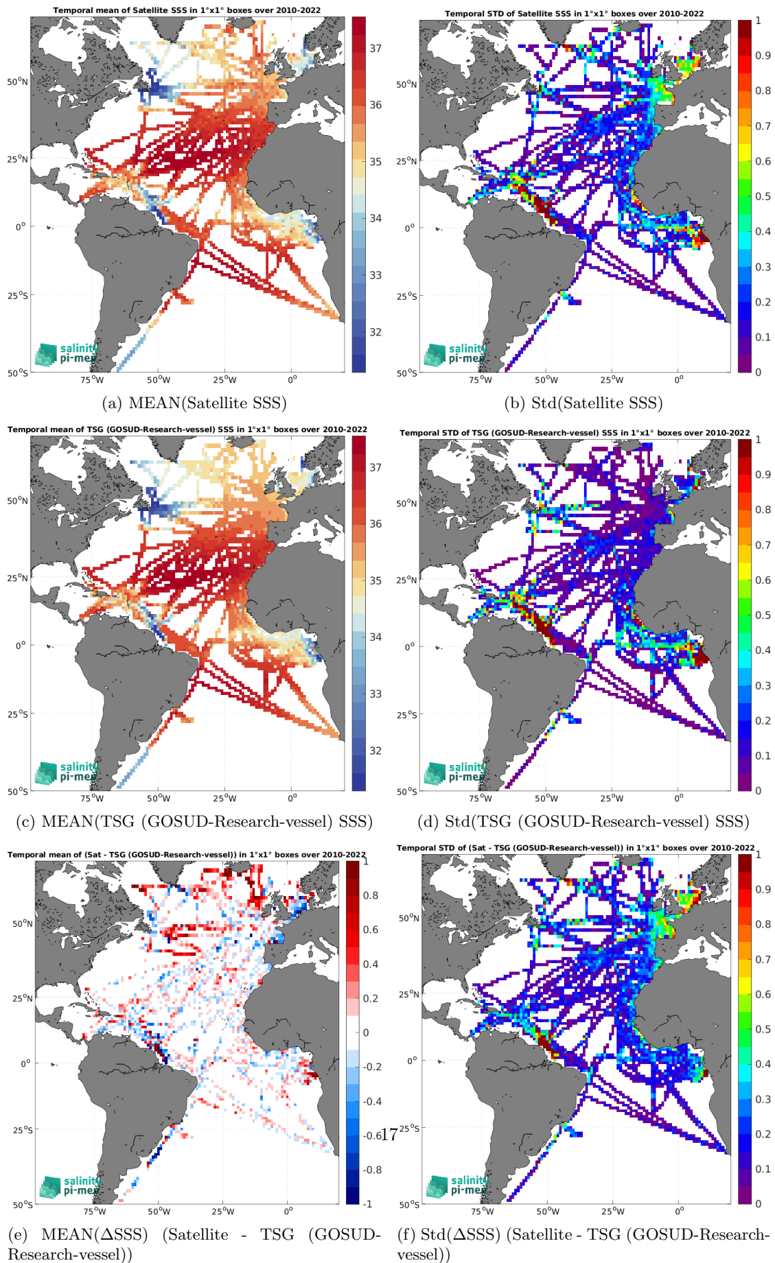
Figure 7: Temporal mean (left) and Std (right) of SSS from SMOS SSS L3 v332 - 9 Days (CATDS-CPDC) (top), TSG (GOSUD-Research-vessel) (middle), and of \Delta SSS (Satellite - TSG (GOSUD-Research-vessel)). Only match-up pairs are used to generate these maps.
