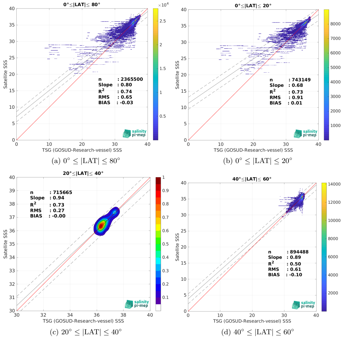
Figure 10: Contour maps of the concentration of SMOS SSS L3 v332 - 9 Days (CATDS-CPDC) SSS (y-axis) versus TSG (GOSUD-Research-vessel) SSS (x-axis) at match-up pairs for different latitude bands. For each plot, the red line shows x=y . The black thin and dashed lines indicate a linear fit through the data cloud and the \pm 95\% confidence levels, respectively. The number match-up pairs n , the slope and R^2 coefficient of the linear fit, the root mean square (RMS) and the mean bias between satellite and in situ data are indicated for each latitude band in each plots.
