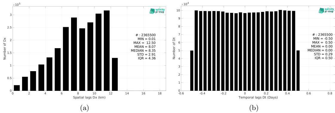
Figure 6: Histograms of the spatial (a) and temporal (b) lags between the location/time of the TSG (GOSUD-Research-vessel) measurement and the date of the corresponding SMOS SSS L3 v332 - 9 Days (CATDS-CPDC) SSS pixel.
