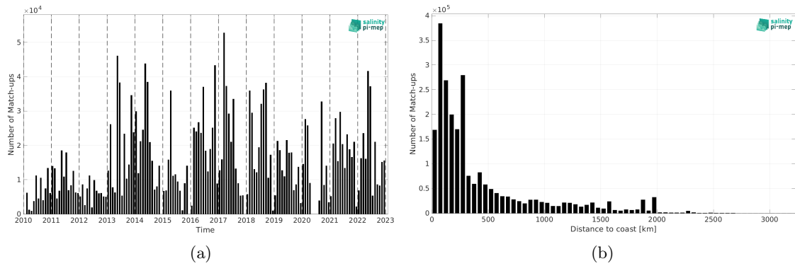
Figure 2: Number of match-ups between TSG (GOSUD-Research-vessel) and SMOS SSS L3 v332 - 9 Days (CATDS-CPDC) SSS as a function of time (a) and as function of the distance to coast (b) over the Atlantic Ocean Pi-MEP region and for the full satellite product period.
