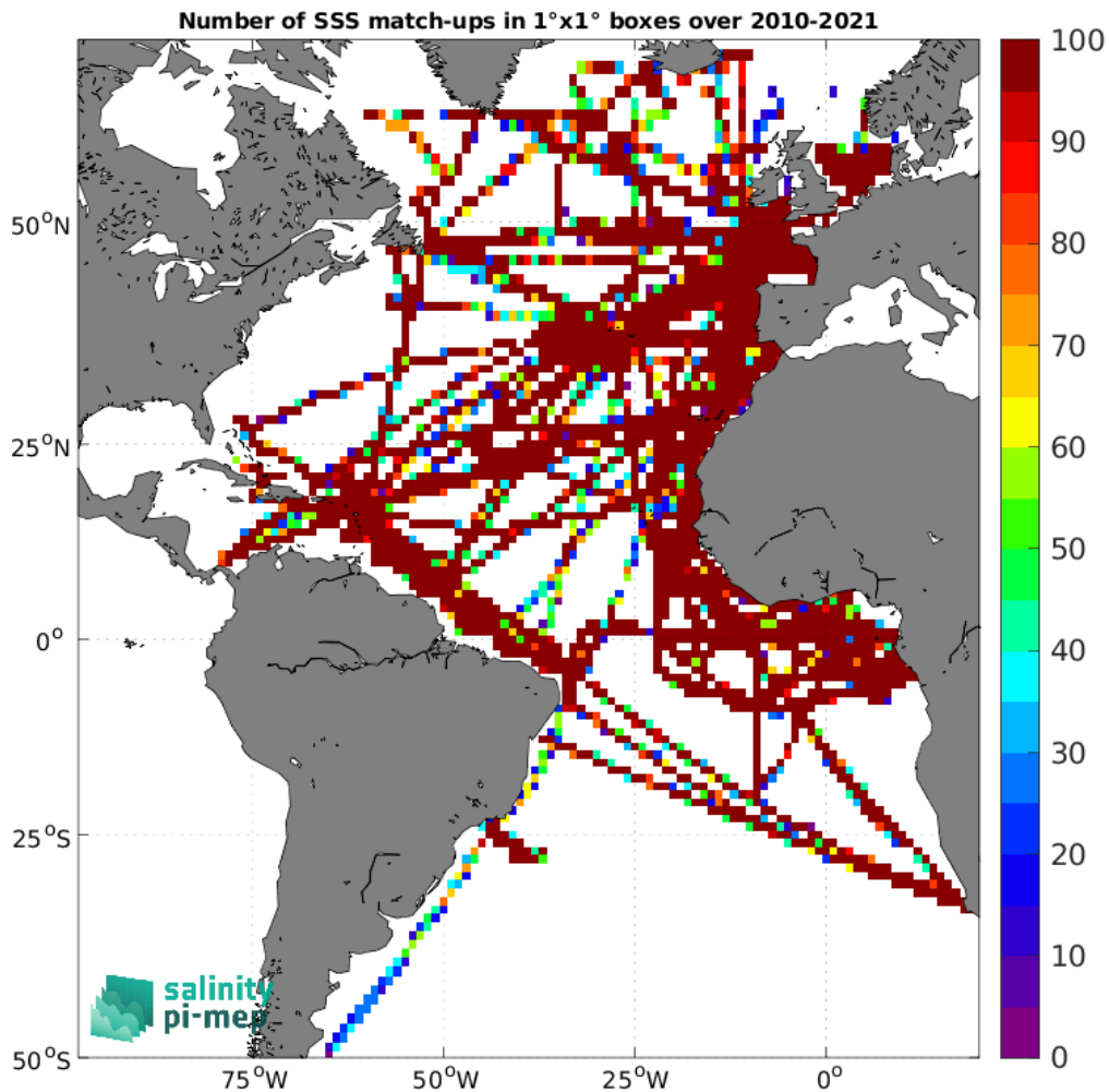
Figure 5: Number of SSS match-ups between TSG (GOSUD-Research-vessel) SSS and the SMOS SSS L3 v332 - 9 Days (CATDS-CPDC) SSS product for the Atlantic Ocean Pi-MEP region over 1^\circ \times 1^\circ boxes and for the full satellite product period.
