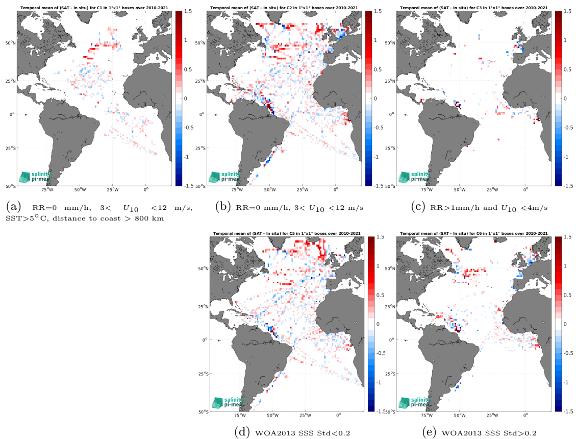
Figure 12: Temporal mean gridded over spatial boxes of size 1^\circ \times 1^\circ of \Delta\text{SSS} (SMOS SSS L3 v332 - 9 Days (CATDS-CPDC) - TSG (GOSUD-Research-vessel)) for 5 different subdatasets corresponding to:RR=0 mm/h, 3 < U_{10} < 12 m/s, SST>5°C, distance to coast > 800 km (a), RR=0 mm/h, 3 < U_{10} < 12 m/s (b), RR>1mm/h and U_{10} < 4 m/s (c), WOA2013 SSS Std<0.2 (d), WOA2013 SSS Std>0.2 (e).
