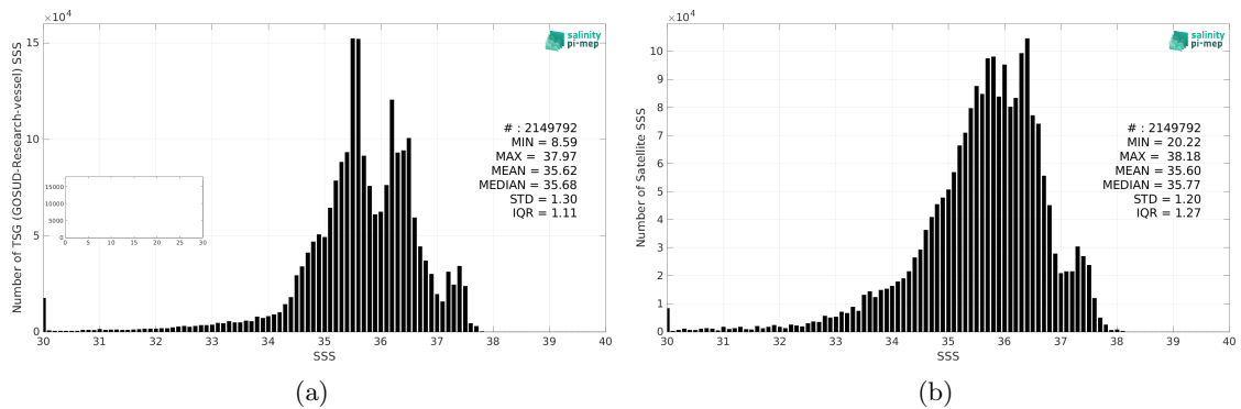
Figure 2: Histograms of SSS from TSG (GOSUD-Research-vessel) (a) and SMOS SSS L3 v332 - 9 Days (CATDS-CPDC) (b) considering all match-up pairs per bins of 0.1 over the Atlantic Ocean Pi-MEP region and for the full satellite product period.
