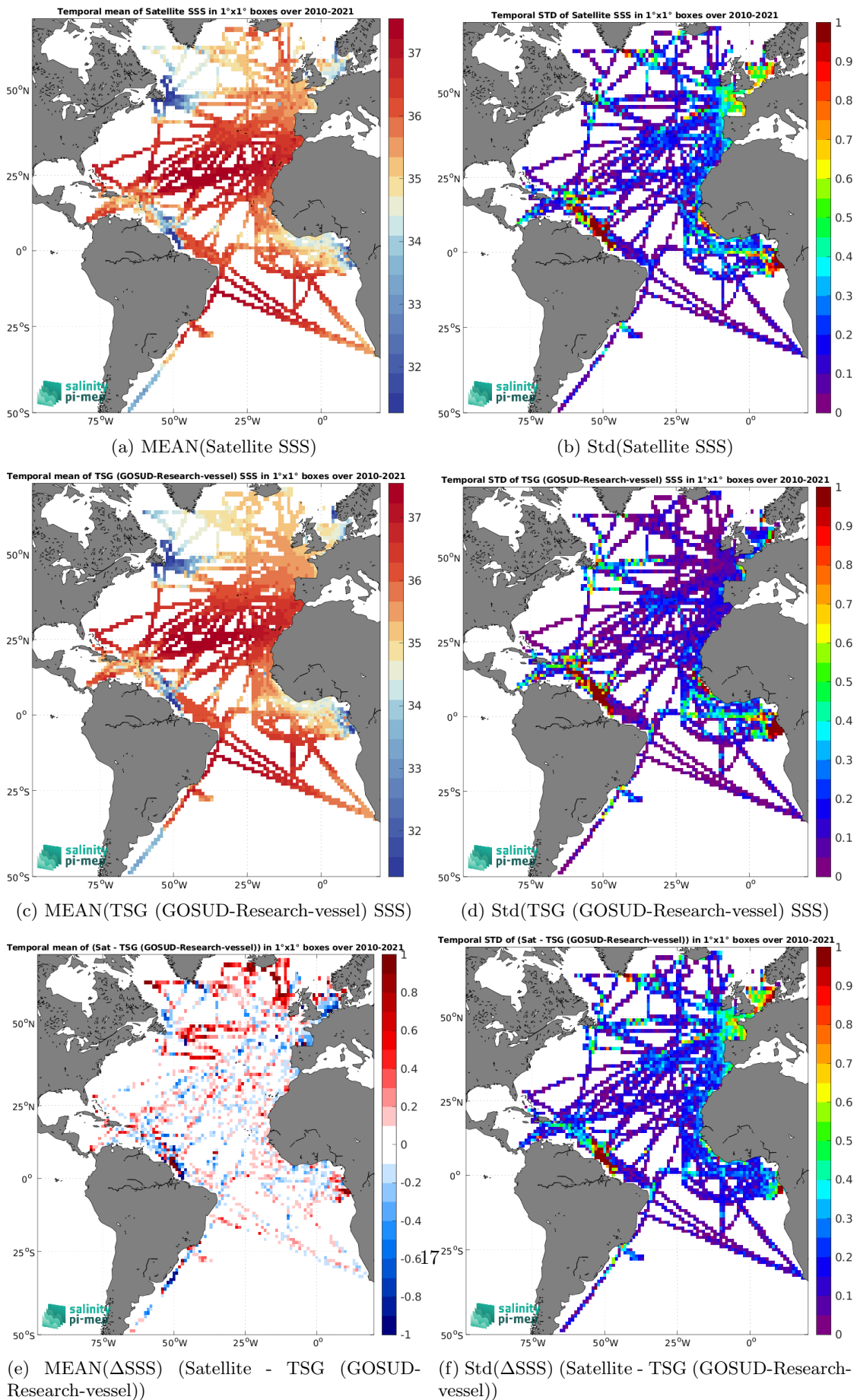
Figure 6: Temporal mean (left) and Std (right) of SSS from SMOS SSS L3 v332 - 9 Days (CATDS-CPDC) (top), TSG (GOSUD-Research-vessel) (middle), and of \Delta SSS (Satellite - TSG (GOSUD-Research-vessel)). Only match-up pairs are used to generate these maps.
