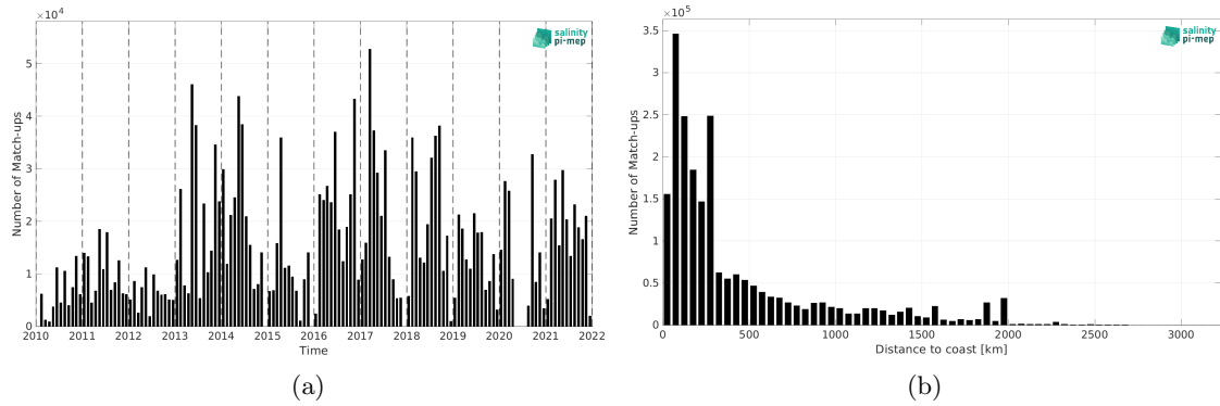
Figure 1: Number of match-ups between TSG (GOSUD-Research-vessel) and SMOS SSS L3 v332 - 9 Days (CATDS-CPDC) SSS as a function of time (a) and as function of the distance to coast (b) over the Atlantic Ocean Pi-MEP region and for the full satellite product period.
