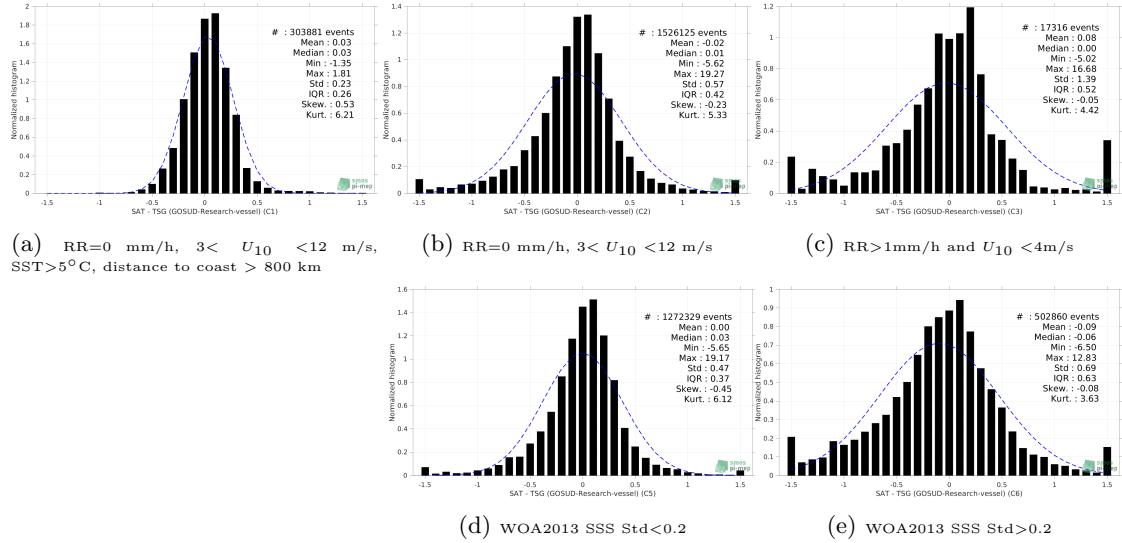
Figure 13: Normalized histogram of \Delta\text{SSS} (SMOS SSS L3 v332 - 9 Days (CATDS-CPDC) - TSG (GOSUD-Research-vessel)) for 5 different subdatasets corresponding to: RR=0 mm/h, 3 < U_{10} < 12 m/s, SST > 5^\circ\text{C} , distance to coast > 800 km (a), RR=0 mm/h, 3 < U_{10} < 12 m/s (b), RR > 1 mm/h and U_{10} < 4 m/s (c), WOA2013 SSS Std < 0.2 (d), WOA2013 SSS Std > 0.2 (e).
