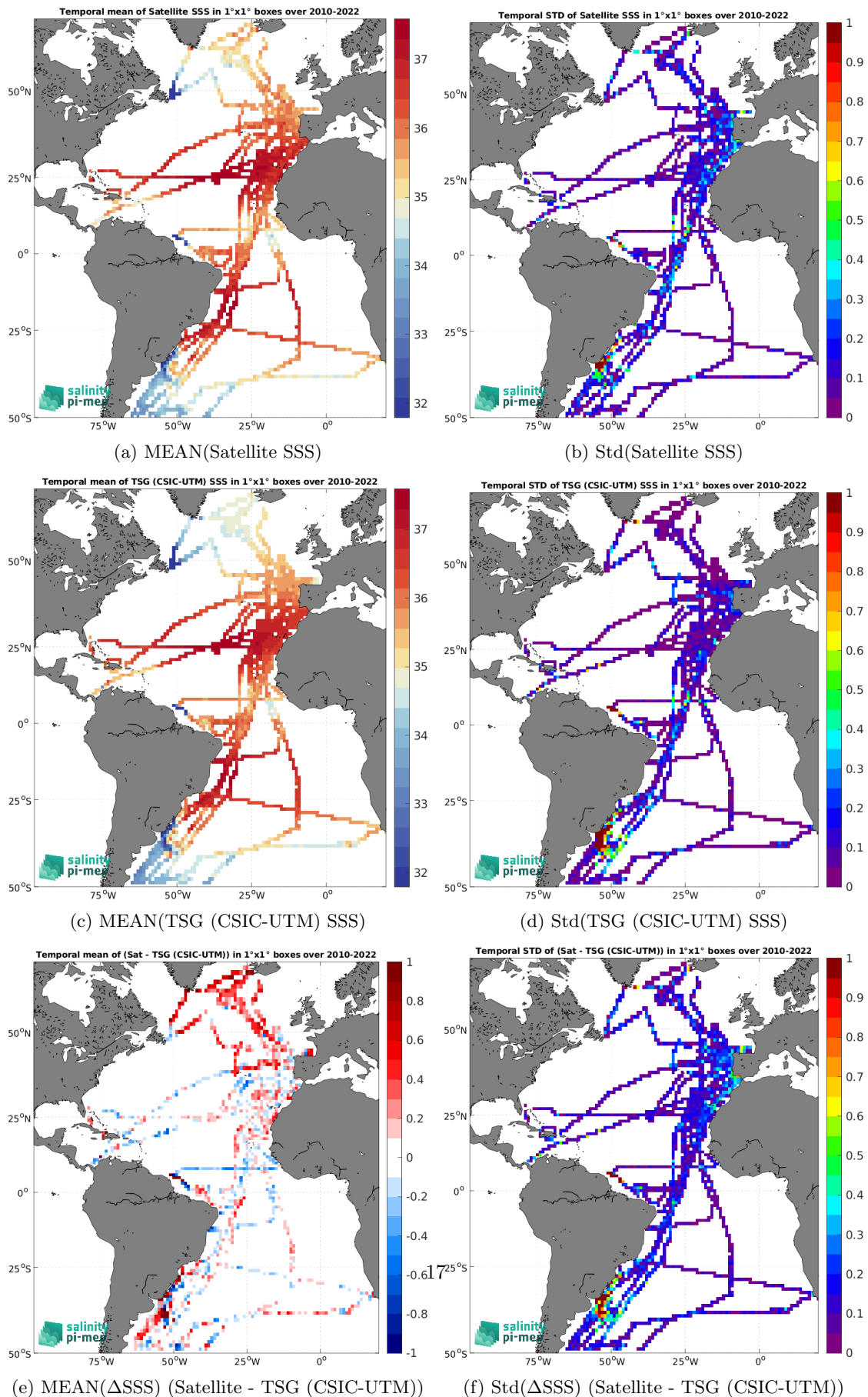
Figure 6: Temporal mean (left) and Std (right) of SSS from SMOS SSS L3 v332 - 9 Days (CATDS-CPDC) (top), TSG (CSIC-UTM) (middle), and of \Delta SSS (Satellite - TSG (CSIC-UTM)). Only match-up pairs are used to generate these maps.
