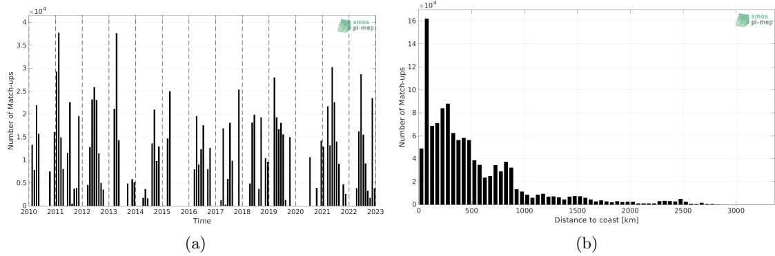
Figure 1: Number of match-ups between TSG (CSIC-UTM) and SMOS SSS L3 v332 - 9 Days (CATDS-CPDC) SSS as a function of time (a) and as function of the distance to coast (b) over the Atlantic Ocean Pi-MEP region and for the full satellite product period.
