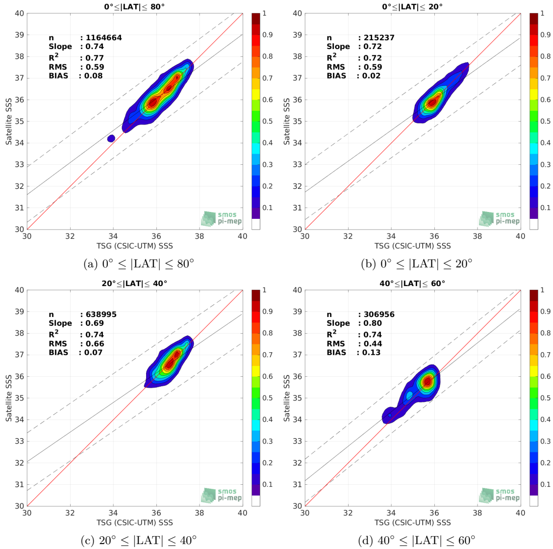
Figure 9: Contour maps of the concentration of SMOS SSS L3 v332 - 9 Days (CATDS-CPDC) SSS (y-axis) versus TSG (CSIC-UTM) SSS (x-axis) at match-up pairs for different latitude bands. For each plot, the red line shows x=y . The black thin and dashed lines indicate a linear fit through the data cloud and the \pm 95\% confidence levels, respectively. The number match-up pairs n , the slope and R^2 coefficient of the linear fit, the root mean square (RMS) and the mean bias between satellite and in situ data are indicated for each latitude band in each plots.
