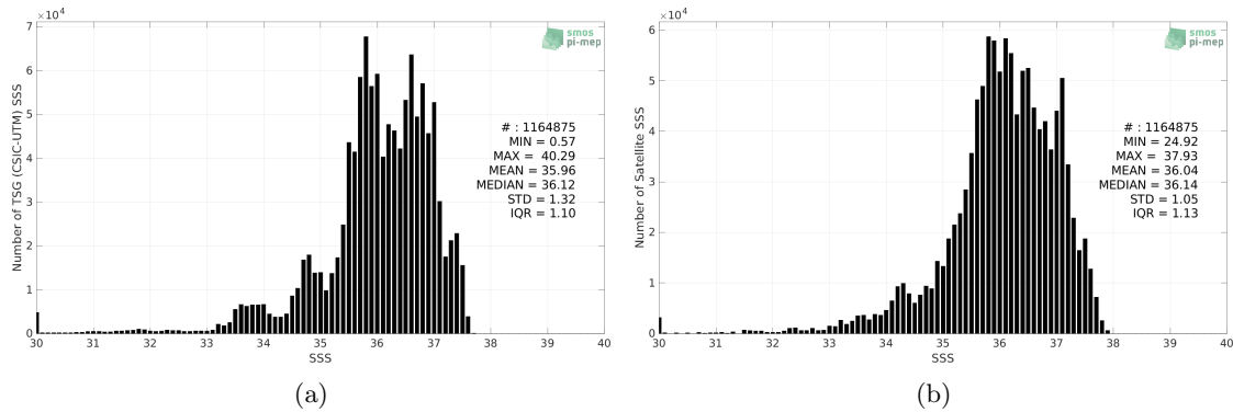
Figure 2: Histograms of SSS from TSG (CSIC-UTM) (a) and SMOS SSS L3 v332 - 9 Days (CATDS-CPDC) (b) considering all match-up pairs per bins of 0.1 over the Atlantic Ocean Pi-MEP region and for the full satellite product period.
