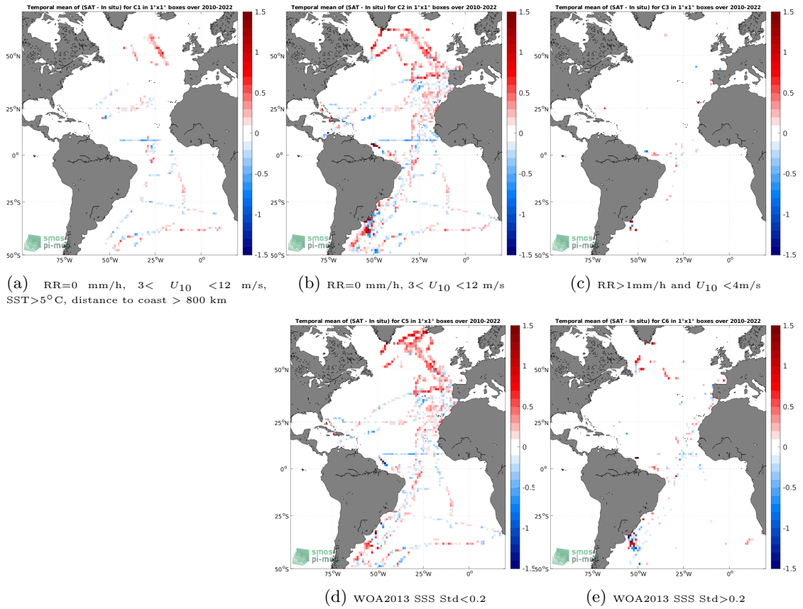
Figure 12: Temporal mean gridded over spatial boxes of size 1^\circ \times 1^\circ of \Delta SSS (SMOS SSS L3 v332 - 9 Days (CATDS-CPDC) - TSG (CSIC-UTM)) for 5 different subdatasets corresponding to:RR=0 mm/h, 3 < U_{10} < 12 m/s, SST >5^\circ\text{C} , distance to coast > 800 km (a), RR=0 mm/h, 3 < U_{10} < 12 m/s (b), RR >1 mm/h and U_{10} < 4 m/s (c), WOA2013 SSS Std <0.2 (d), WOA2013 SSS Std >0.2 (e).
