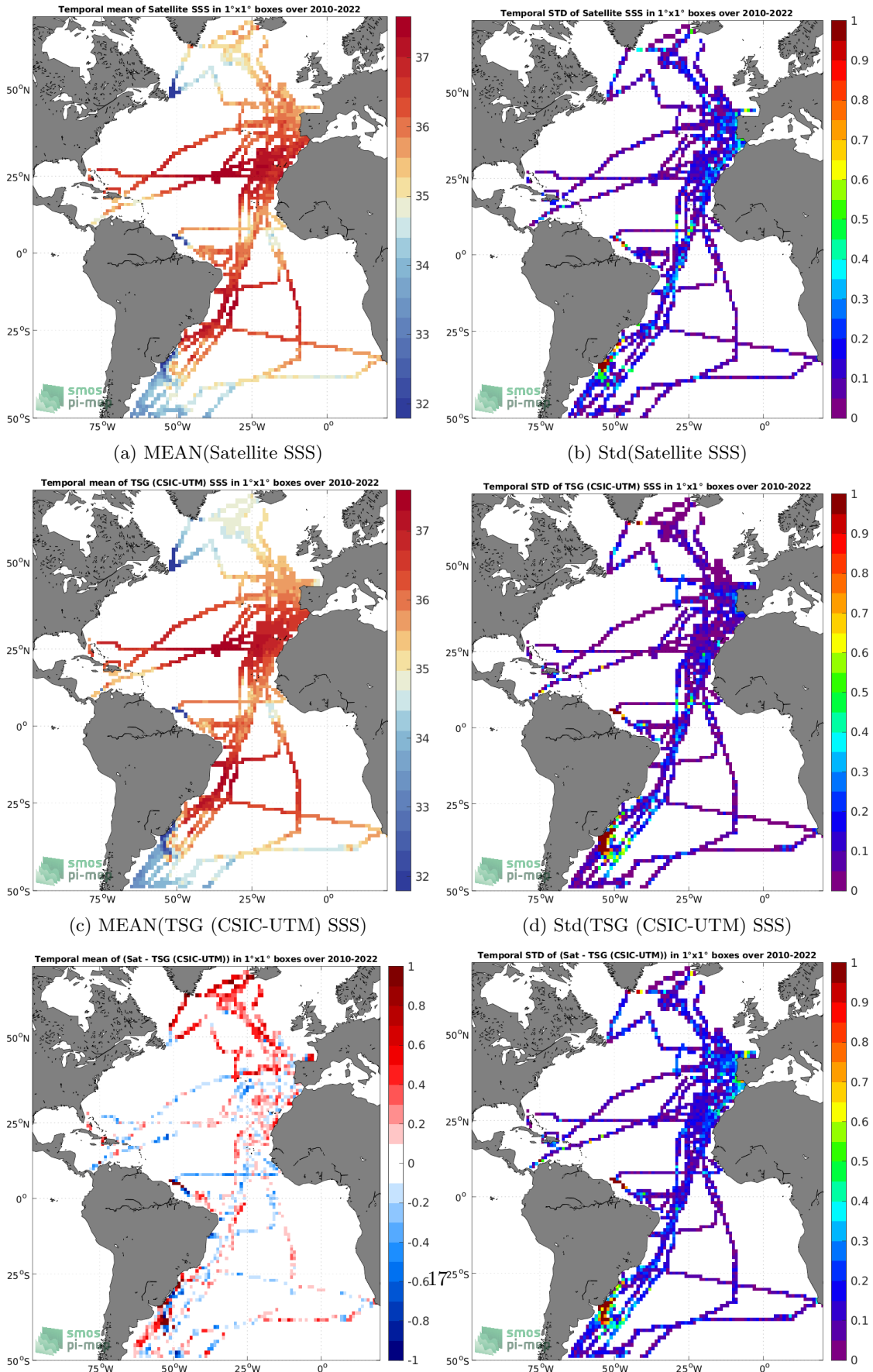
(e) MEAN( \Delta SSS) (Satellite - TSG (CSIC-UTM)) (f) Std( \Delta SSS) (Satellite - TSG (CSIC-UTM)) Figure 6: Temporal mean (left) and Std (right) of SSS from SMOS SSS L3 v332 - 9 Days (CATDS-CPDC) (top), TSG (CSIC-UTM) (middle), and of \Delta SSS (Satellite - TSG (CSIC-UTM)). Only match-up pairs are used to generate these maps.
