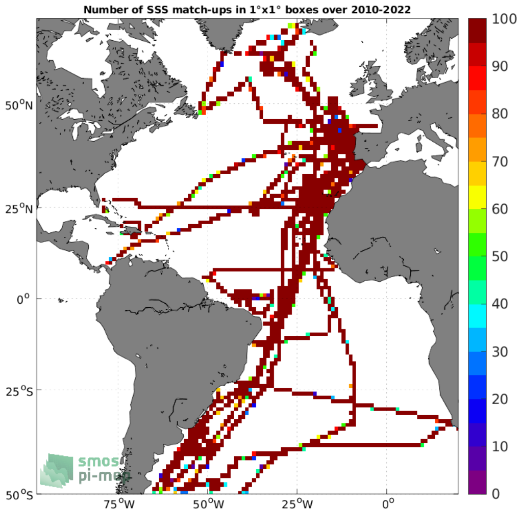
Figure 4: Number of SSS match-ups between TSG (CSIC-UTM) SSS and the SMOS SSS L3 v332 - 9 Days (CATDS-CPDC) SSS product for the Atlantic Ocean Pi-MEP region over 1°x1° boxes and for the full satellite product period.
