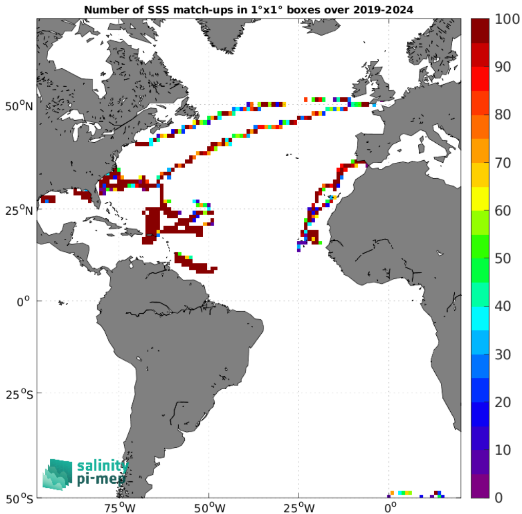
Figure 5: Number of SSS match-ups between Saildrone SSS and the SMOS SSS L3 v332 - 9 Days (CATDS-CPDC) SSS product for the Atlantic Ocean Pi-MEP region over 1°×1° boxes and for the full satellite product period.
