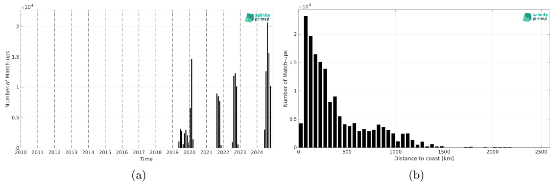
Figure 2: Number of match-ups between Saildrone and SMOS SSS L3 v332 - 9 Days (CATDS-CPDC) SSS as a function of time (a) and as function of the distance to coast (b) over the Atlantic Ocean Pi-MEP region and for the full satellite product period.
