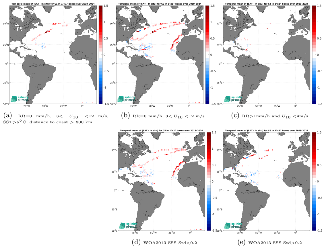
Figure 14: Temporal mean gridded over spatial boxes of size 1^\circ \times 1^\circ of \Delta\text{SSS} (SMOS SSS L3 v332 - 9 Days (CATDS-CPDC) - Sailability) for 5 different subdatasets corresponding to:RR=0 mm/h, 3 < U_{10} < 12 m/s, SST>5°C, distance to coast > 800 km (a), RR=0 mm/h, 3 < U_{10} < 12 m/s (b), RR>1mm/h and U_{10} < 4 m/s (c), WOA2013 SSS Std<0.2 (d), WOA2013 SSS Std>0.2 (e).
