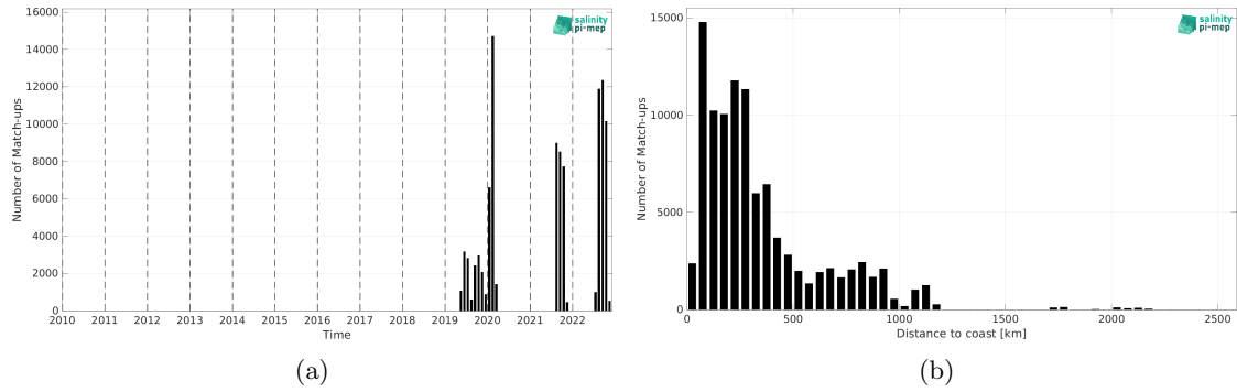
Figure 2: Number of match-ups between Saildrone and SMOS SSS L3 v332 - 9 Days (CATDS-CPDC) SSS as a function of time (a) and as function of the distance to coast (b) over the Atlantic Ocean Pi-MEP region and for the full satellite product period.
