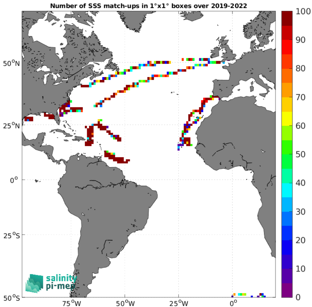
Figure 5: Number of SSS match-ups between Saildrone SSS and the SMOS SSS L3 v332 - 9 Days (CATDS-CPDC) SSS product for the Atlantic Ocean Pi-MEP region over 1^\circ \times 1^\circ boxes and for the full satellite product period.
