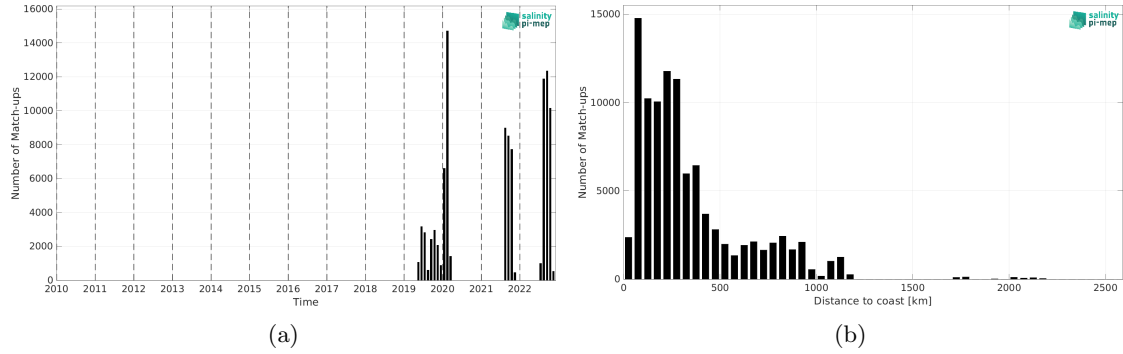
Figure 1: Number of match-ups between Saildrone and SMOS SSS L3 v332 - 9 Days (CATDS-CPDC) SSS as a function of time (a) and as function of the distance to coast (b) over the Atlantic Ocean Pi-MEP region and for the full satellite product period.
