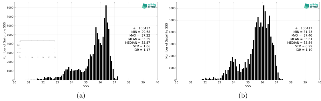
Figure 2: Histograms of SSS from Saildrone (a) and SMOS SSS L3 v332 - 9 Days (CATDS-CPDC) (b) considering all match-up pairs per bins of 0.1 over the Atlantic Ocean Pi-MEP region and for the full satellite product period.
