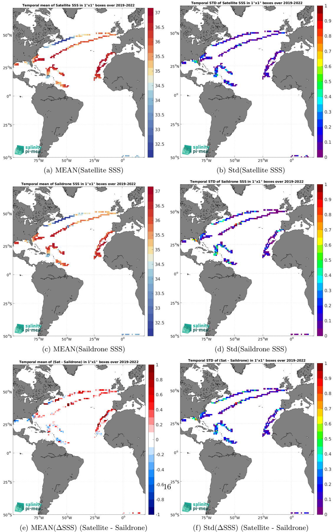
Figure 6: Temporal mean (left) and Std (right) of SSS from SMOS SSS L3 v332 - 9 Days (CATDS-CPDC) (top), Saildrones (middle), and of \Delta SSS (Satellite - Saildrones). Only match-up pairs are used to generate these maps.
