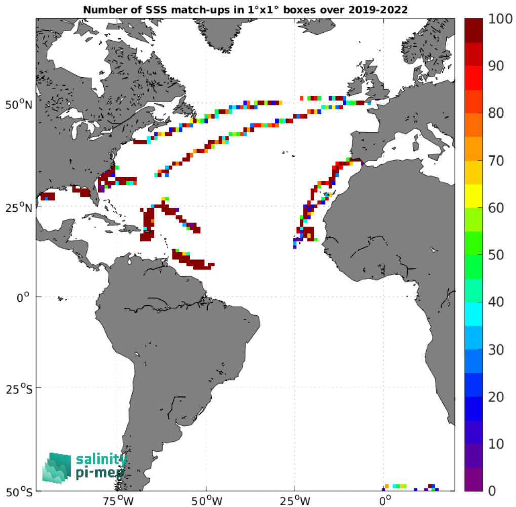
Figure 4: Number of SSS match-ups between Saildrone SSS and the SMOS SSS L3 v332 - 9 Days (CATDS-CPDC) SSS product for the Atlantic Ocean Pi-MEP region over 1°×1° boxes and for the full satellite product period.
