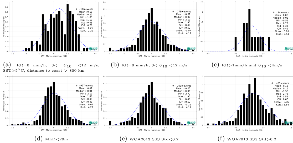
Figure 15: Normalized histogram of \Delta\text{SSS} (SMOS SSS L3 v332 - 9 Days (CATDS-CPDC) - Marine mammals) for 6 different subdatasets corresponding to: RR=0 mm/h, 3 < U_{10} < 12 m/s, SST>5°C, distance to coast > 800 km (a), RR=0 mm/h, 3 < U_{10} < 12 m/s (b), RR>1mm/h and U_{10} < 4 m/s (c), MLD<20m (d), WOA2013 SSS Std<0.2 (e), WOA2013 SSS Std>0.2 (f).
