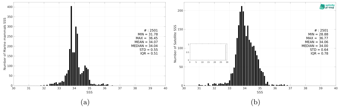
Figure 3: Histograms of SSS from Marine mammals (a) and SMOS SSS L3 v332 - 9 Days (CATDS-CPDC) (b) considering all match-up pairs per bins of 0.1 over the Atlantic Ocean Pi-MEP region and for the full satellite product period.
