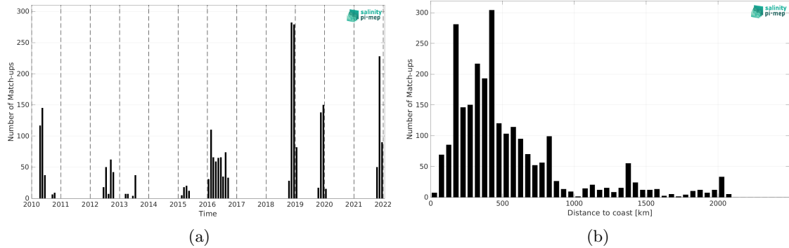
Figure 2: Number of match-ups between Marine mammals and SMOS SSS L3 v332 - 9 Days (CATDS-CPDC) SSS as a function of time (a) and as function of the distance to coast (b) over the Atlantic Ocean Pi-MEP region and for the full satellite product period.
