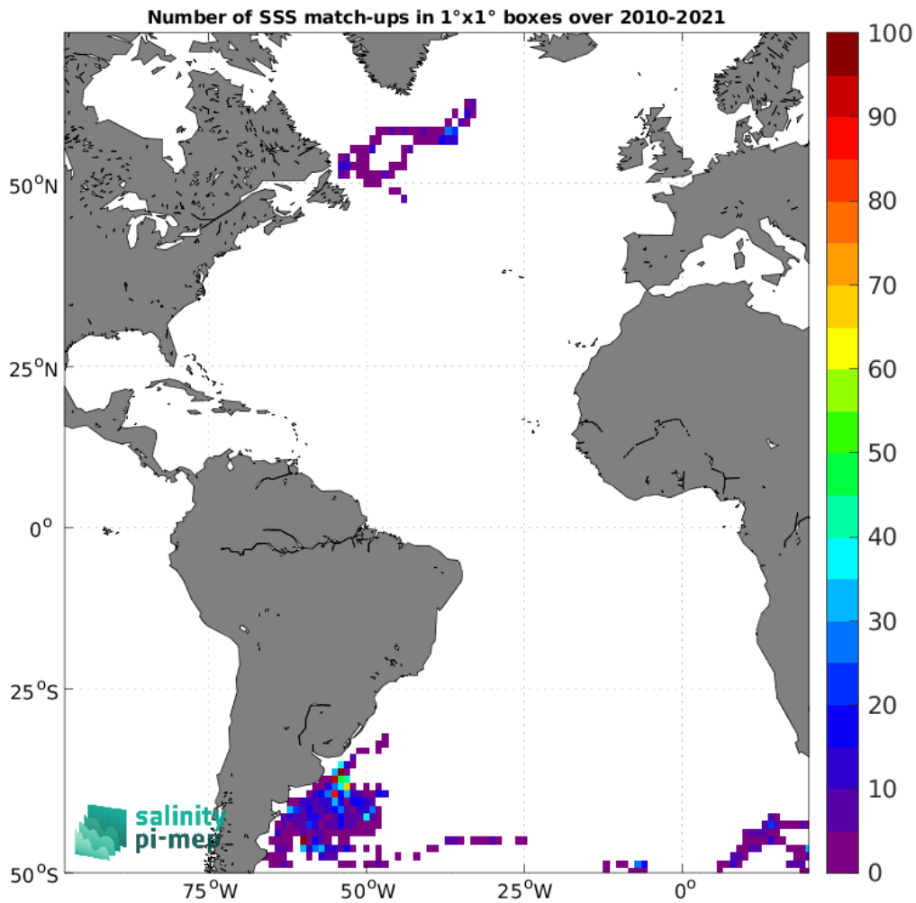
Figure 5: Number of SSS match-ups between Marine mammals SSS and the SMOS SSS L3 v332 - 9 Days (CATDS-CPDC) SSS product for the Atlantic Ocean Pi-MEP region over 1°×1° boxes and for the full satellite product period.
