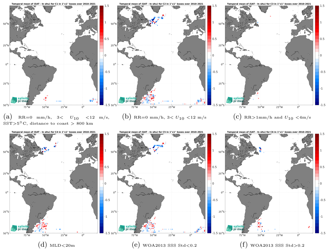
Figure 14: Temporal mean gridded over spatial boxes of size 1^\circ \times 1^\circ of \Delta SSS (SMOS SSS L3 v332 - 9 Days (CATDS-CPDC) - Marine mammals) for 6 different subdatasets corresponding to:RR=0 mm/h, 3 < U_{10} < 12 m/s, SST >5^\circ C, distance to coast > 800 km (a), RR=0 mm/h, 3 < U_{10} < 12 m/s (b), RR >1 mm/h and U_{10} < 4 m/s (c),MLD <20 m (d),WOA2013 SSS Std <0.2 (e),WOA2013 SSS Std >0.2 (f).
