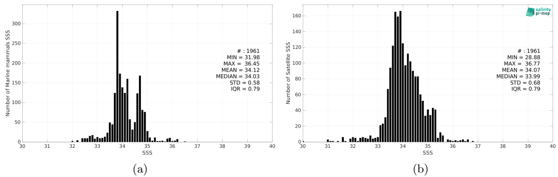
Figure 2: Histograms of SSS from Marine mammals (a) and SMOS SSS L3 v332 - 9 Days (CATDS-CPDC) (b) considering all match-up pairs per bins of 0.1 over the Atlantic Ocean Pi-MEP region and for the full satellite product period.
