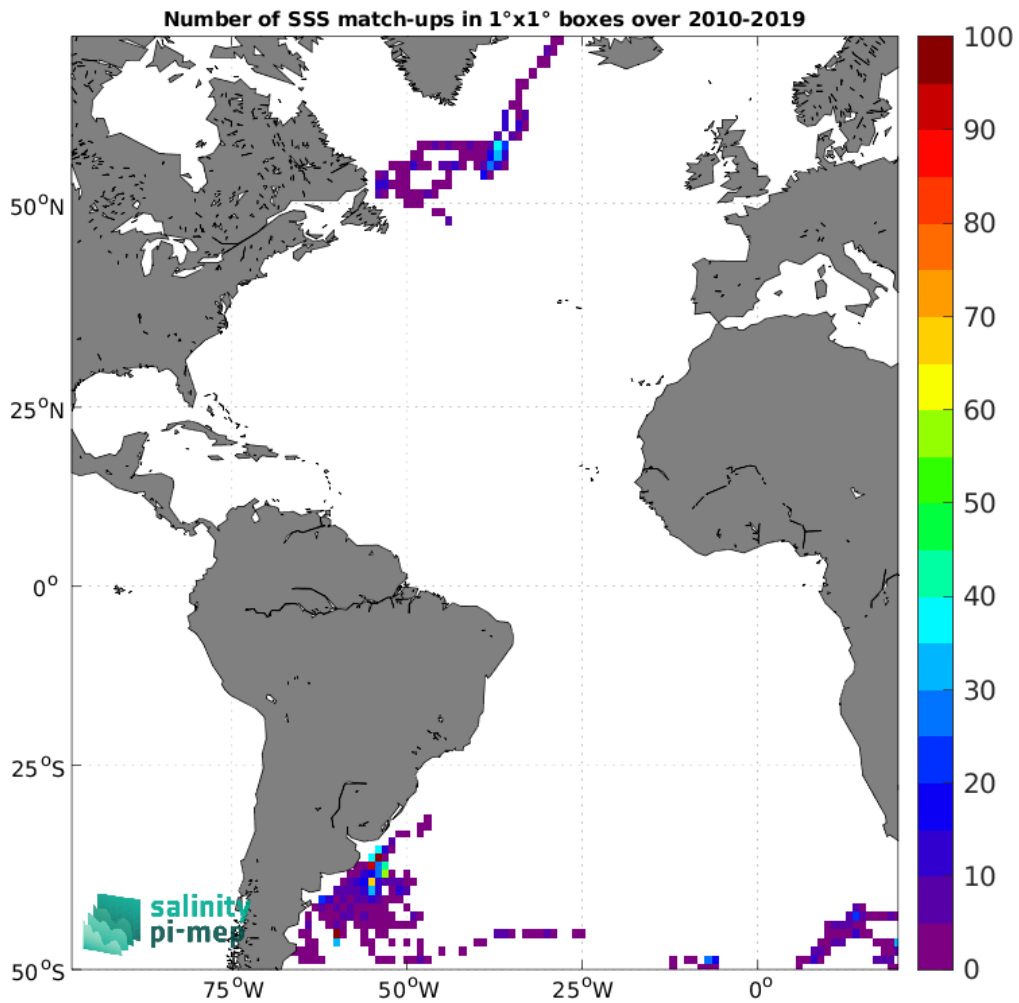
Figure 4: Number of SSS match-ups between Marine mammals SSS and the SMOS SSS L3 v332 - 9 Days (CATDS-CPDC) SSS product for the Atlantic Ocean Pi-MEP region over 1°×1° boxes and for the full satellite product period.
