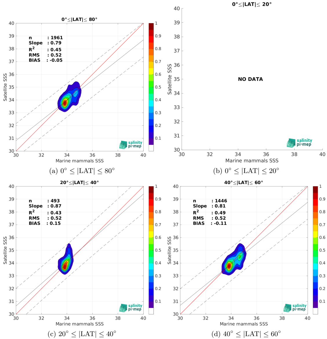
Figure 9: Contour maps of the concentration of SMOS SSS L3 v332 - 9 Days (CATDS-CPDC) SSS (y-axis) versus Marine mammals SSS (x-axis) at match-up pairs for different latitude bands. For each plot, the red line shows x=y . The black thin and dashed lines indicate a linear fit through the data cloud and the \pm 95\% confidence levels, respectively. The number match-up pairs n , the slope and R^2 coefficient of the linear fit, the root mean square (RMS) and the mean bias between satellite and in situ data are indicated for each latitude band in each plots.
