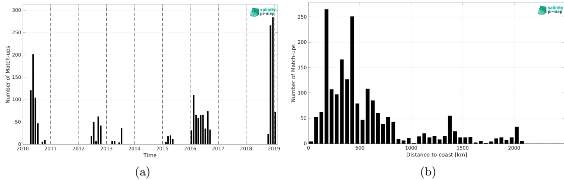
Figure 1: Number of match-ups between Marine mammals and SMOS SSS L3 v332 - 9 Days (CATDS-CPDC) SSS as a function of time (a) and as function of the distance to coast (b) over the Atlantic Ocean Pi-MEP region and for the full satellite product period.
