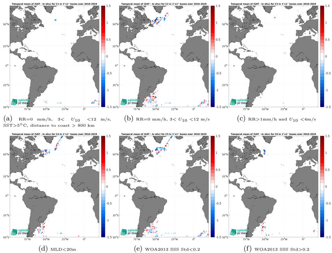
Figure 12: Temporal mean gridded over spatial boxes of size 1^\circ \times 1^\circ of \Delta SSS (SMOS SSS L3 v332 - 9 Days (CATDS-CPDC) - Marine mammals) for 6 different subdatasets corresponding to:RR=0 mm/h, 3 < U_{10} < 12 m/s, SST >5^\circ C, distance to coast > 800 km (a), RR=0 mm/h, 3 < U_{10} < 12 m/s (b), RR >1 mm/h and U_{10} < 4 m/s (c),MLD <20 m (d),WOA2013 SSS Std <0.2 (e),WOA2013 SSS Std >0.2 (f).
