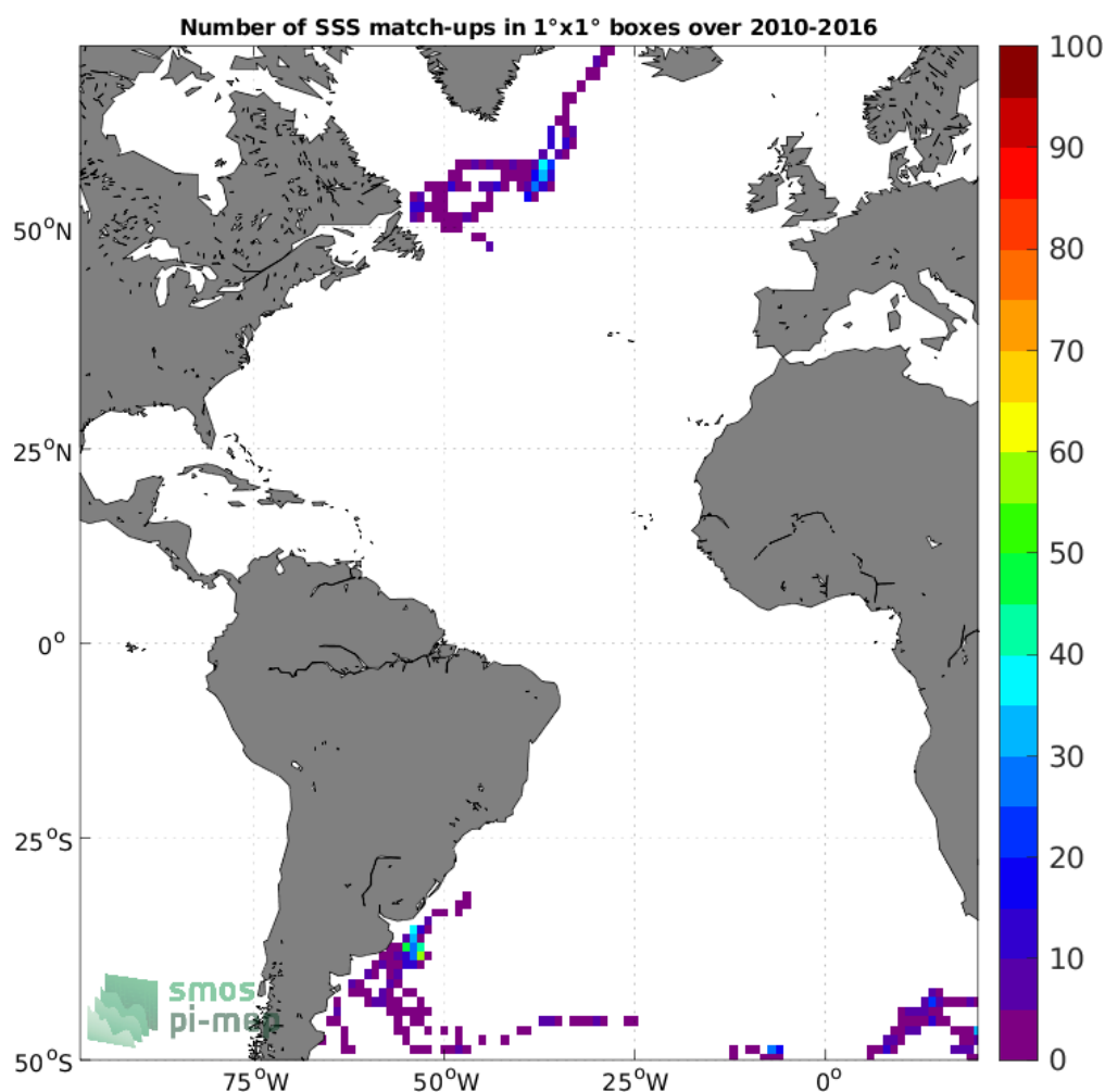
Figure 4: Number of SSS match-ups between Marine mammals SSS and the SMOS SSS L3 v332 - 9 Days (CATDS-CPDC) SSS product for the Atlantic Ocean Pi-MEP region over 1°x1° boxes and for the full satellite product period.
