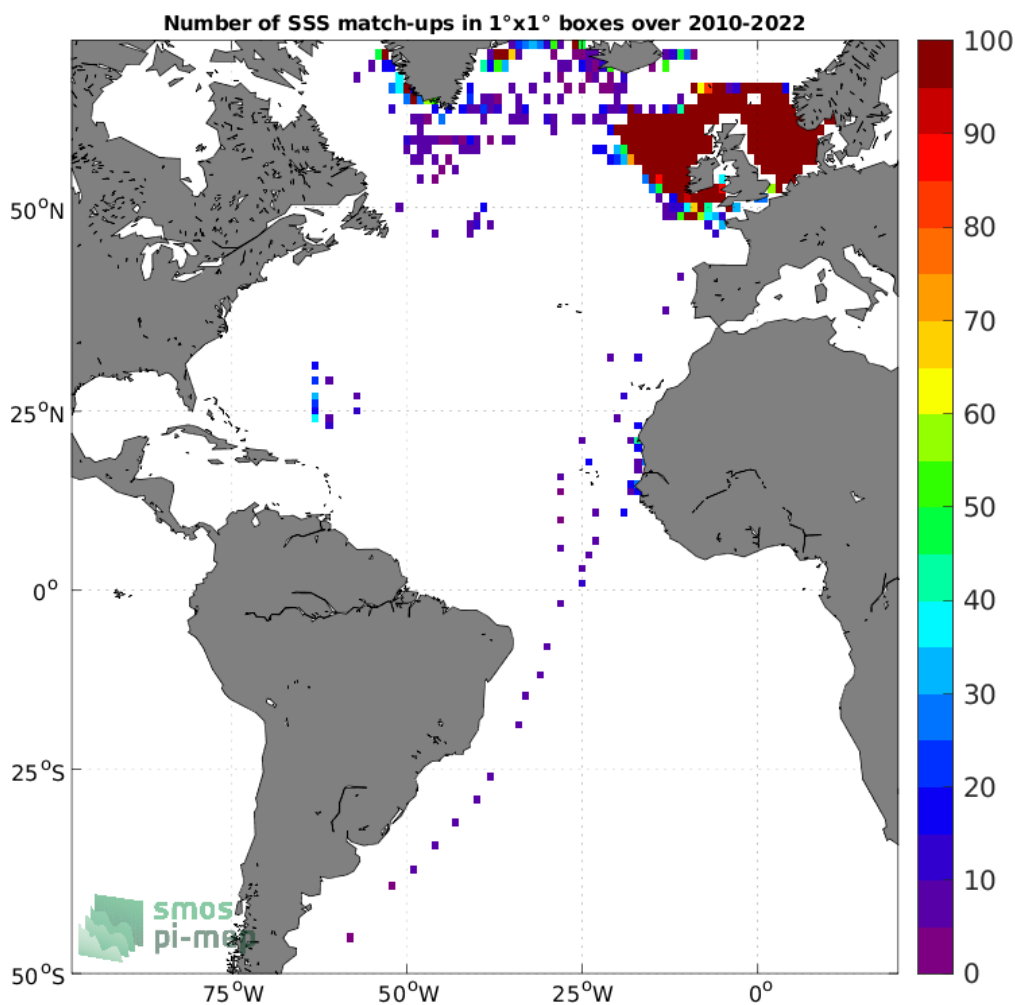
Figure 4: Number of SSS match-ups between ICES SSS and the SMOS SSS L3 v332 - 9 Days (CATDS-CPDC) SSS product for the Atlantic Ocean Pi-MEP region over 1°x1° boxes and for the full satellite product period.
