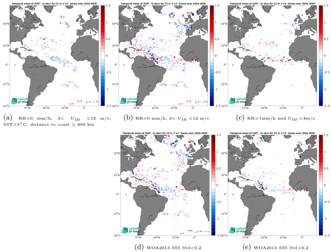
Figure 11: Temporal mean gridded over spatial boxes of size 1^\circ \times 1^\circ of \Delta\text{SSS} (SMOS SSS L3 v332 - 9 Days (CATDS-CPDC) - Surface drifters) for 5 different subdatasets corresponding to:RR=0 mm/h, 3 < U_{10} < 12 m/s, SST >5^\circ\text{C} , distance to coast > 800 km (a), RR=0 mm/h, 3 < U_{10} < 12 m/s (b), RR >1 mm/h and U_{10} < 4 m/s (c), WOA2013 SSS Std <0.2 (d), WOA2013 SSS Std >0.2 (e).
