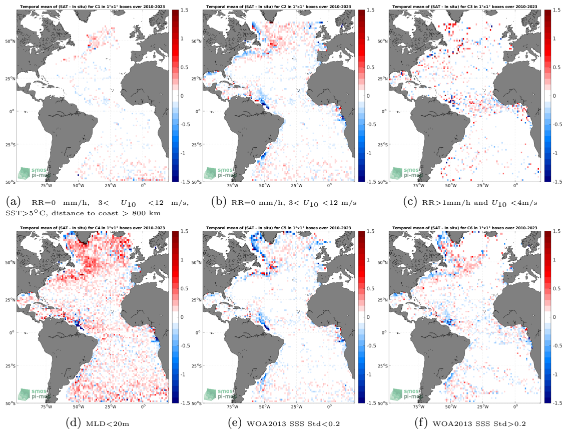
Figure 12: Temporal mean gridded over spatial boxes of size 1^\circ \times 1^\circ of \Delta SSS (SMOS SSS L3 v332 - 9 Days (CATDS-CPDC) - Argo) for 6 different subdatasets corresponding to:RR=0 mm/h, 3 < U_{10} < 12 m/s, SST >5^\circ C, distance to coast > 800 km (a), RR=0 mm/h, 3 < U_{10} < 12 m/s (b), RR >1 mm/h and U_{10} < 4 m/s (c),MLD <20 m (d),WOA2013 SSS Std <0.2 (e),WOA2013 SSS Std >0.2 (f).
