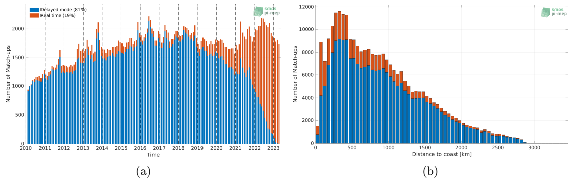
Figure 1: Number of match-ups between Argo and SMOS SSS L3 v332 - 9 Days (CATDS-CPDC) SSS as a function of time (a) and as function of the distance to coast (b) over the Atlantic Ocean Pi-MEP region and for the full satellite product period.
