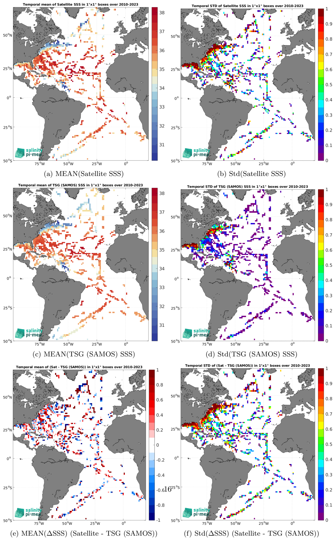
Figure 6: Temporal mean (left) and Std (right) of SSS from SMOS SSS L2Q v331 - 0.25 Deg (CATDS-CPDC) (top), TSG (SAMOS) (middle), and of \Delta SSS (Satellite - TSG (SAMOS)). Only match-up pairs are used to generate these maps.
