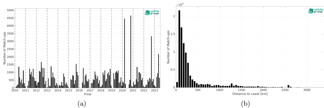
Figure 1: Number of match-ups between TSG (SAMOS) and SMOS SSS L2Q v331 - 0.25 Deg (CATDS-CPDC) SSS as a function of time (a) and as function of the distance to coast (b) over the Atlantic Ocean Pi-MEP region and for the full satellite product period.
