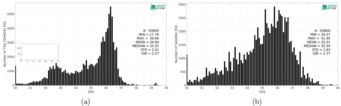
Figure 2: Histograms of SSS from TSG (SAMOS) (a) and SMOS SSS L2Q v331 - 0.25 Deg (CATDS-CPDC) (b) considering all match-up pairs per bins of 0.1 over the Atlantic Ocean Pi-MEP region and for the full satellite product period.
