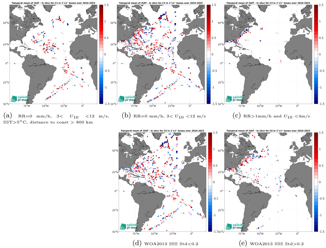
Figure 12: Temporal mean gridded over spatial boxes of size 1^\circ \times 1^\circ of \Delta SSS (SMOS SSS L2Q v331 - 0.25 Deg (CATDS-CPDC) - TSG (SAMOS)) for 5 different subdatasets corresponding to:RR=0 mm/h, 3 < U_{10} < 12 m/s, SST >5^\circ\text{C} , distance to coast > 800 km (a), RR=0 mm/h, 3 < U_{10} < 12 m/s (b), RR >1 mm/h and U_{10} < 4 m/s (c), WOA2013 SSS Std <0.2 (d), WOA2013 SSS Std >0.2 (e).
