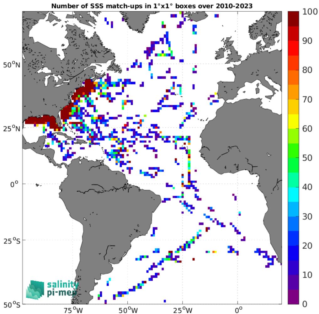
Figure 4: Number of SSS match-ups between TSG (SAMOS) SSS and the SMOS SSS L2Q v331 - 0.25 Deg (CATDS-CPDC) SSS product for the Atlantic Ocean Pi-MEP region over 1^\circ \times 1^\circ boxes and for the full satellite product period.
