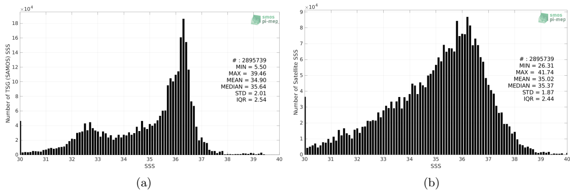
Figure 2: Histograms of SSS from TSG (SAMOS) (a) and SMOS SSS L2Q v331 - 0.25 Deg (CATDS-CPDC) (b) considering all match-up pairs per bins of 0.1 over the Atlantic Ocean Pi-MEP region and for the full satellite product period.
