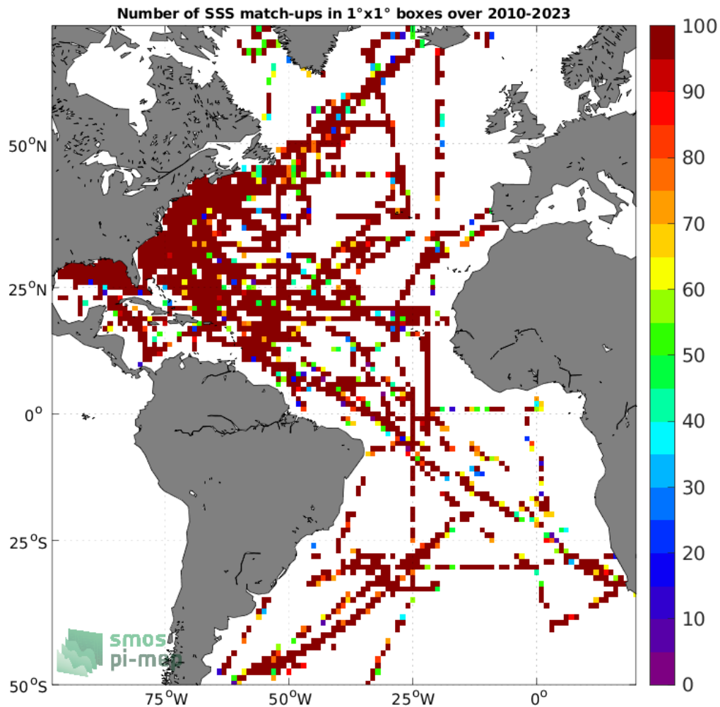
Figure 4: Number of SSS match-ups between TSG (SAMOS) SSS and the SMOS SSS L2Q v331 - 0.25 Deg (CATDS-CPDC) SSS product for the Atlantic Ocean Pi-MEP region over 1°x1° boxes and for the full satellite product period.
