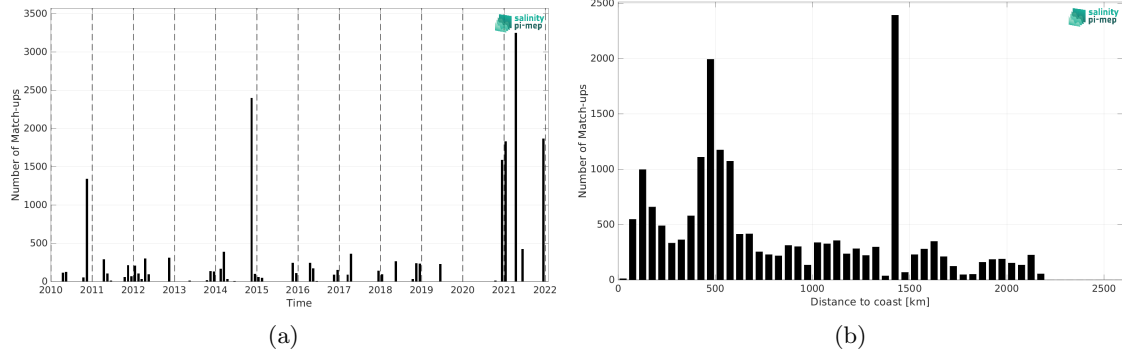
Figure 1: Number of match-ups between TSG (Polarstern) and SMOS SSS L2Q v331 - 0.25 Deg (CATDS-CPDC) SSS as a function of time (a) and as function of the distance to coast (b) over the Atlantic Ocean Pi-MEP region and for the full satellite product period.
