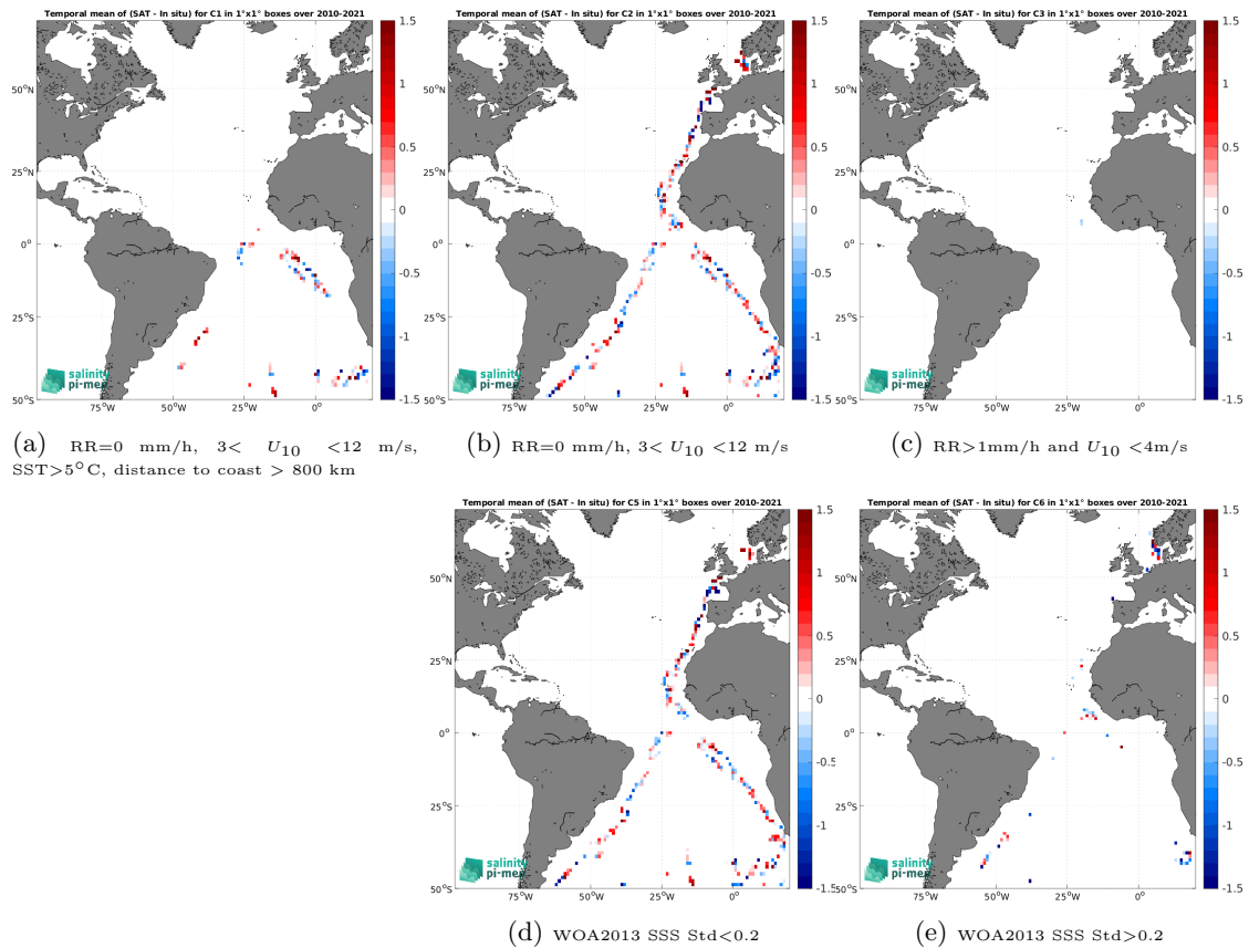
Figure 12: Temporal mean gridded over spatial boxes of size 1^\circ \times 1^\circ of \Delta\text{SSS} (SMOS SSS L2Q v331 - 0.25 Deg (CATDS-CPDC) - TSG (Polarstern)) for 5 different subdatasets corresponding to:RR=0 mm/h, 3 < U_{10} < 12 m/s, SST >5^\circ\text{C} , distance to coast > 800 km (a), RR=0 mm/h, 3 < U_{10} < 12 m/s (b), RR >1 mm/h and U_{10} < 4 m/s (c), WOA2013 SSS Std <0.2 (d), WOA2013 SSS Std >0.2 (e).
