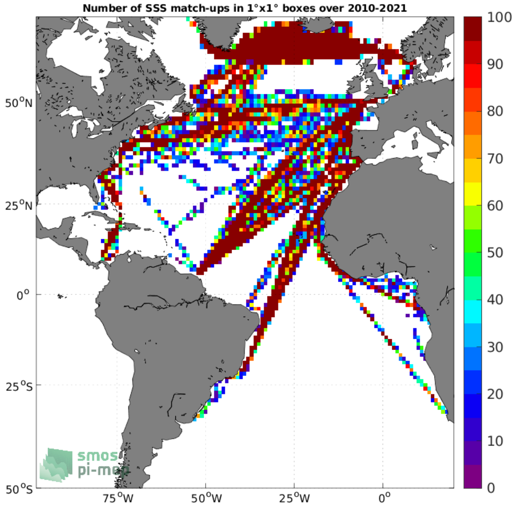
Figure 4: Number of SSS match-ups between TSG (LEGOS-DM) SSS and the SMOS SSS L2Q v331 - 0.25 Deg (CATDS-CPDC) SSS product for the Atlantic Ocean Pi-MEP region over 1°x1° boxes and for the full satellite product period.
