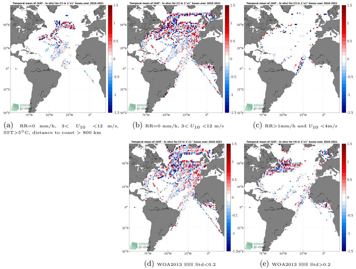
Figure 12: Temporal mean gridded over spatial boxes of size 1^\circ \times 1^\circ of \Delta SSS (SMOS SSS L2Q v331 - 0.25 Deg (CATDS-CPDC) - TSG (LEGOS-DM)) for 5 different subdatasets corresponding to:RR=0 mm/h, 3 < U_{10} < 12 m/s, SST >5^\circ\text{C} , distance to coast > 800 km (a), RR=0 mm/h, 3 < U_{10} < 12 m/s (b), RR >1 mm/h and U_{10} < 4 m/s (c), WOA2013 SSS Std <0.2 (d), WOA2013 SSS Std >0.2 (e).
