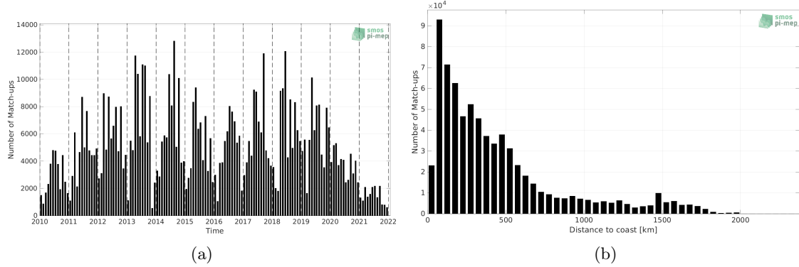
Figure 1: Number of match-ups between TSG (LEGOS-DM) and SMOS SSS L2Q v331 - 0.25 Deg (CATDS-CPDC) SSS as a function of time (a) and as function of the distance to coast (b) over the Atlantic Ocean Pi-MEP region and for the full satellite product period.
