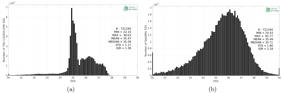
Figure 2: Histograms of SSS from TSG (LEGOS-DM) (a) and SMOS SSS L2Q v331 - 0.25 Deg (CATDS-CPDC) (b) considering all match-up pairs per bins of 0.1 over the Atlantic Ocean Pi-MEP region and for the full satellite product period.
