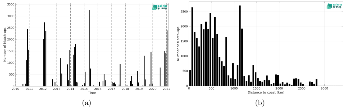
Figure 1: Number of match-ups between TSG (GOSUD-Sailing-ship) and SMOS SSS L2Q v331 - 0.25 Deg (CATDS-CPDC) SSS as a function of time (a) and as function of the distance to coast (b) over the Atlantic Ocean Pi-MEP region and for the full satellite product period.
