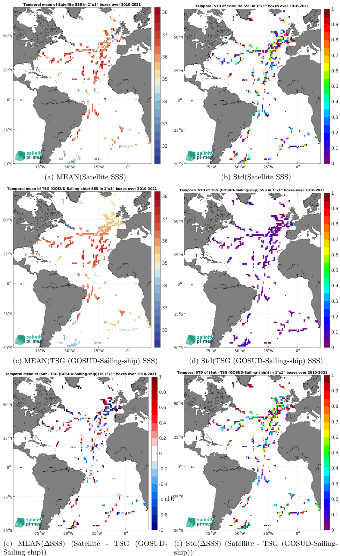
Figure 6: Temporal mean (left) and Std (right) of SSS from SMOS SSS L2Q v331 - 0.25 Deg (CATDS-CPDC) (top), TSG (GOSUD-Sailing-ship) (middle), and of \Delta SSS (Satellite - TSG (GOSUD-Sailing-ship)). Only match-up pairs are used to generate these maps.
