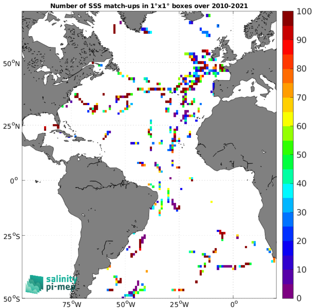
Figure 4: Number of SSS match-ups between TSG (GOSUD-Sailing-ship) SSS and the SMOS SSS L2Q v331 - 0.25 Deg (CATDS-CPDC) SSS product for the Atlantic Ocean Pi-MEP region over 1°x1° boxes and for the full satellite product period.
