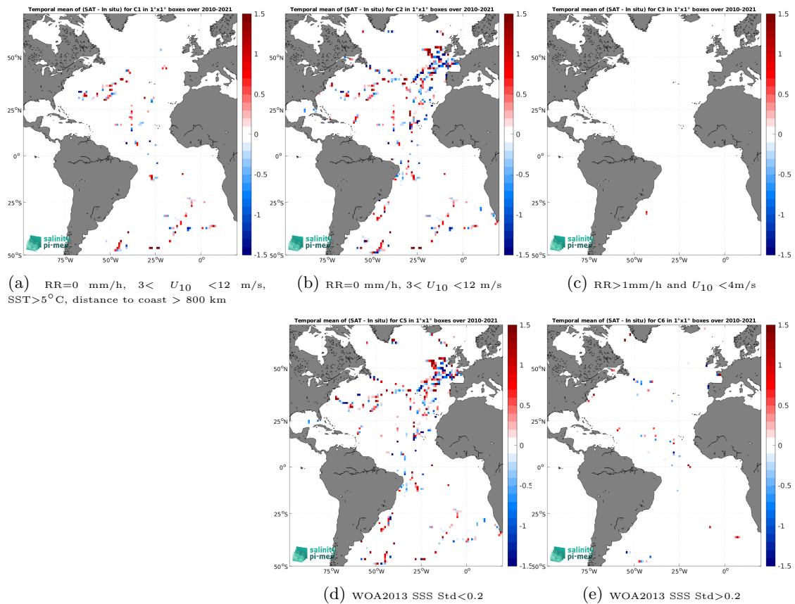
Figure 12: Temporal mean gridded over spatial boxes of size 1^\circ \times 1^\circ of \Delta\text{SSS} (SMOS SSS L2Q v331 - 0.25 Deg (CATDS-CPDC) - TSG (GOSUD-Sailing-ship)) for 5 different subdatasets corresponding to:RR=0 mm/h, 3 < U_{10} < 12 m/s, SST>5°C, distance to coast > 800 km (a), RR=0 mm/h, 3 < U_{10} < 12 m/s (b), RR>1mm/h and U_{10} < 4 m/s (c), WOA2013 SSS Std<0.2 (d), WOA2013 SSS Std>0.2 (e).
