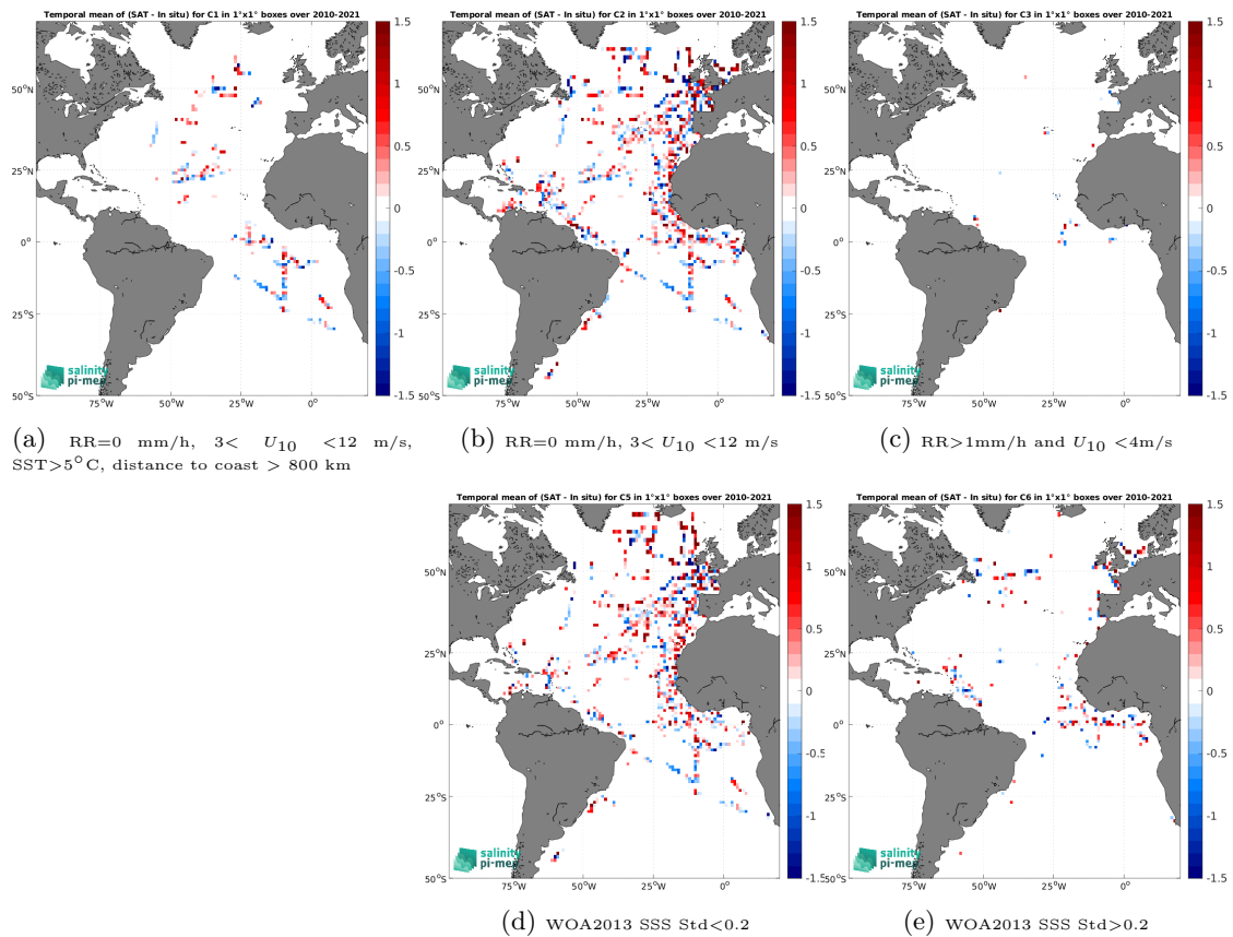
Figure 12: Temporal mean gridded over spatial boxes of size 1^\circ \times 1^\circ of \Delta\text{SSS} (SMOS SSS L2Q v331 - 0.25 Deg (CATDS-CPDC) - TSG (GOSUD-Research-vessel)) for 5 different subdatasets corresponding to:RR=0 mm/h, 3 < U_{10} < 12 m/s, SST >5^\circ\text{C} , distance to coast > 800 km (a), RR=0 mm/h, 3 < U_{10} < 12 m/s (b), RR >1 mm/h and U_{10} < 4 m/s (c), WOA2013 SSS Std <0.2 (d), WOA2013 SSS Std >0.2 (e).
