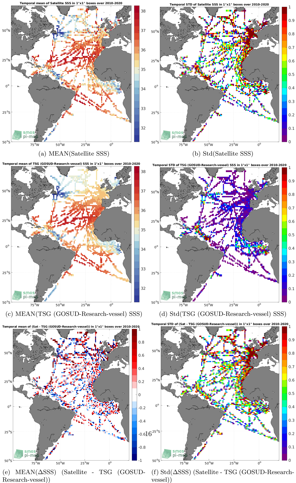
Figure 6: Temporal mean (left) and Std (right) of SSS from SMOS SSS L2Q v331 - 0.25 Deg (CATDS-CPDC) (top), TSG (GOSUD-Research-vessel) (middle), and of \Delta SSS (Satellite - TSG (GOSUD-Research-vessel)). Only match-up pairs are used to generate these maps.
