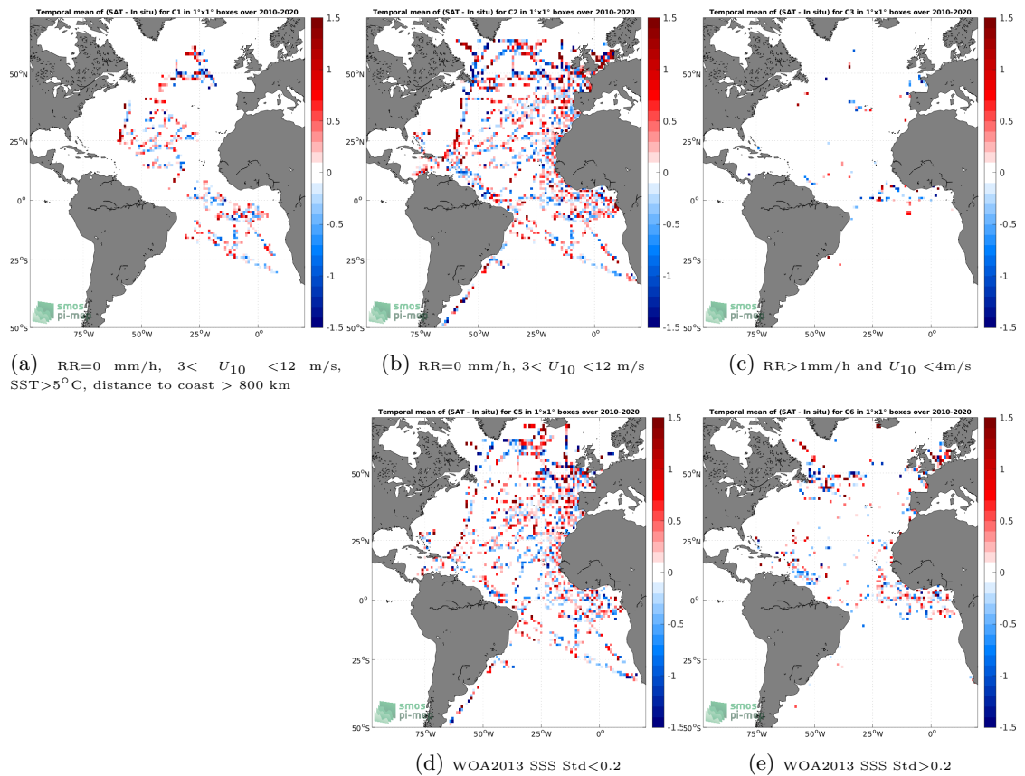
Figure 12: Temporal mean gridded over spatial boxes of size 1^\circ \times 1^\circ of \Delta\text{SSS} (SMOS SSS L2Q v331 - 0.25 Deg (CATDS-CPDC) - TSG (GOSUD-Research-vessel)) for 5 different subdatasets corresponding to:RR=0 mm/h, 3 < U_{10} < 12 m/s, SST>5°C, distance to coast > 800 km (a), RR=0 mm/h, 3 < U_{10} < 12 m/s (b), RR>1mm/h and U_{10} < 4 m/s (c), WOA2013 SSS Std<0.2 (d), WOA2013 SSS Std>0.2 (e).
