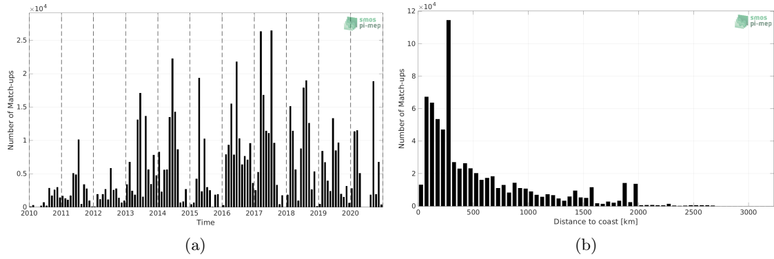
Figure 1: Number of match-ups between TSG (GOSUD-Research-vessel) and SMOS SSS L2Q v331 - 0.25 Deg (CATDS-CPDC) SSS as a function of time (a) and as function of the distance to coast (b) over the Atlantic Ocean Pi-MEP region and for the full satellite product period.
