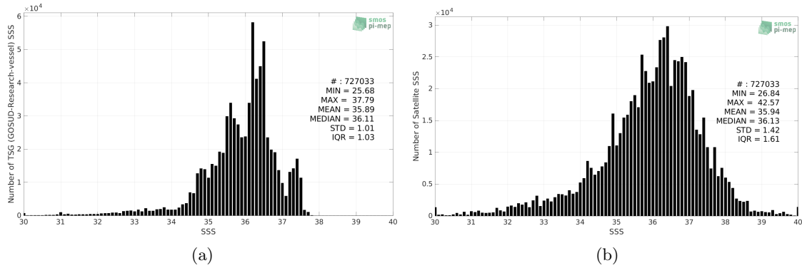
Figure 2: Histograms of SSS from TSG (GOSUD-Research-vessel) (a) and SMOS SSS L2Q v331 - 0.25 Deg (CATDS-CPDC) (b) considering all match-up pairs per bins of 0.1 over the Atlantic Ocean Pi-MEP region and for the full satellite product period.
