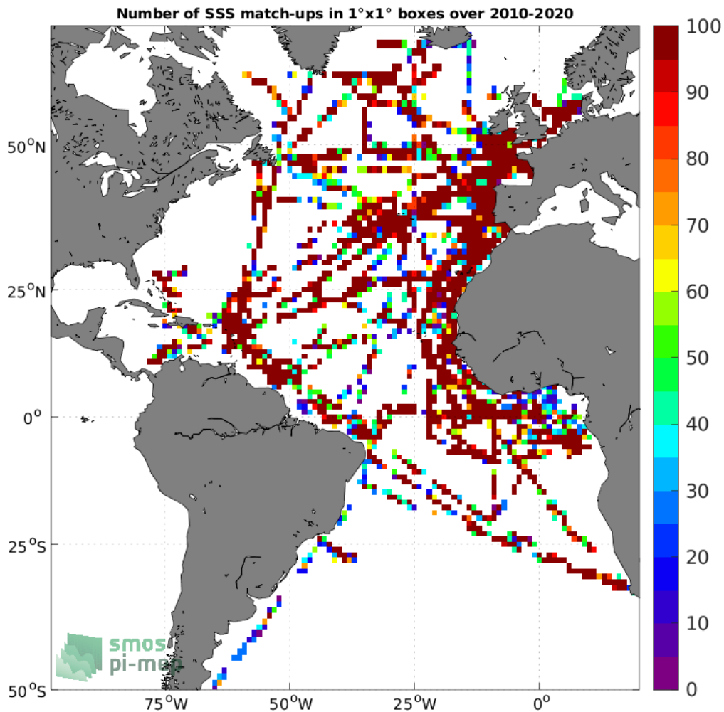
Figure 4: Number of SSS match-ups between TSG (GOSUD-Research-vessel) SSS and the SMOS SSS L2Q v331 - 0.25 Deg (CATDS-CPDC) SSS product for the Atlantic Ocean Pi-MEP region over 1°x1° boxes and for the full satellite product period.
