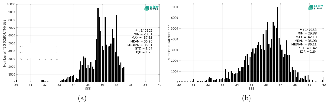
Figure 2: Histograms of SSS from TSG (CSIC-UTM) (a) and SMOS SSS L2Q v331 - 0.25 Deg (CATDS-CPDC) (b) considering all match-up pairs per bins of 0.1 over the Atlantic Ocean Pi-MEP region and for the full satellite product period.
