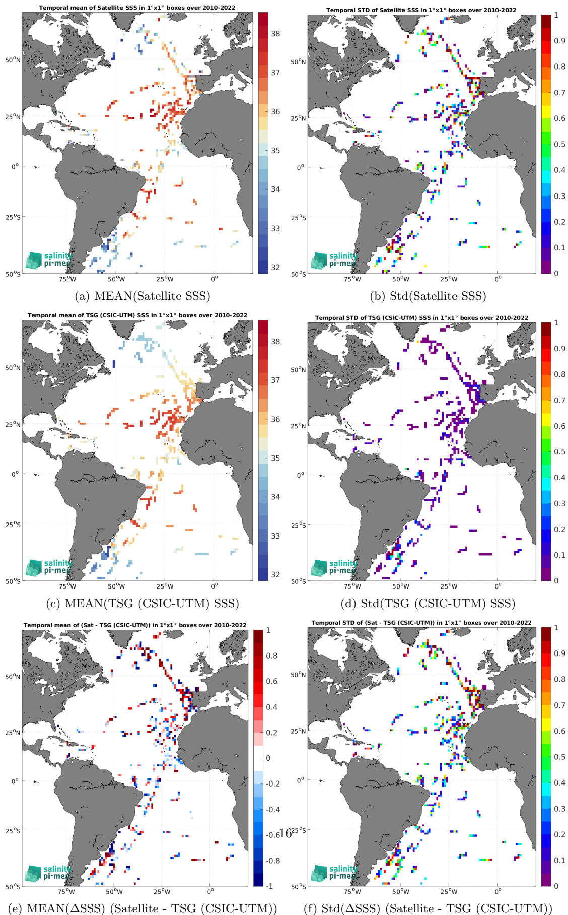
Figure 6: Temporal mean (left) and Std (right) of SSS from SMOS SSS L2Q v331 - 0.25 Deg (CATDS-CPDC) (top), TSG (CSIC-UTM) (middle), and of \Delta SSS (Satellite - TSG (CSIC-UTM)). Only match-up pairs are used to generate these maps.
