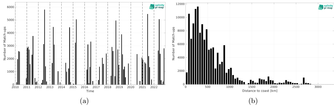
Figure 1: Number of match-ups between TSG (CSIC-UTM) and SMOS SSS L2Q v331 - 0.25 Deg (CATDS-CPDC) SSS as a function of time (a) and as function of the distance to coast (b) over the Atlantic Ocean Pi-MEP region and for the full satellite product period.
