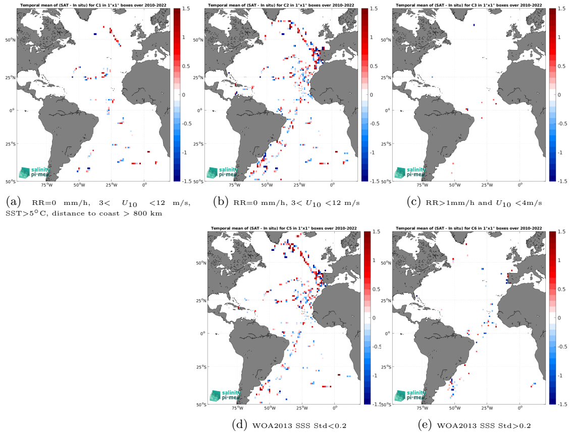
Figure 12: Temporal mean gridded over spatial boxes of size 1^\circ \times 1^\circ of \Delta SSS (SMOS SSS L2Q v331 - 0.25 Deg (CATDS-CPDC) - TSG (CSIC-UTM)) for 5 different subdatasets corresponding to:RR=0 mm/h, 3 < U_{10} < 12 m/s, SST >5^\circ\text{C} , distance to coast > 800 km (a), RR=0 mm/h, 3 < U_{10} < 12 m/s (b), RR >1 mm/h and U_{10} < 4 m/s (c), WOA2013 SSS Std <0.2 (d), WOA2013 SSS Std >0.2 (e).
