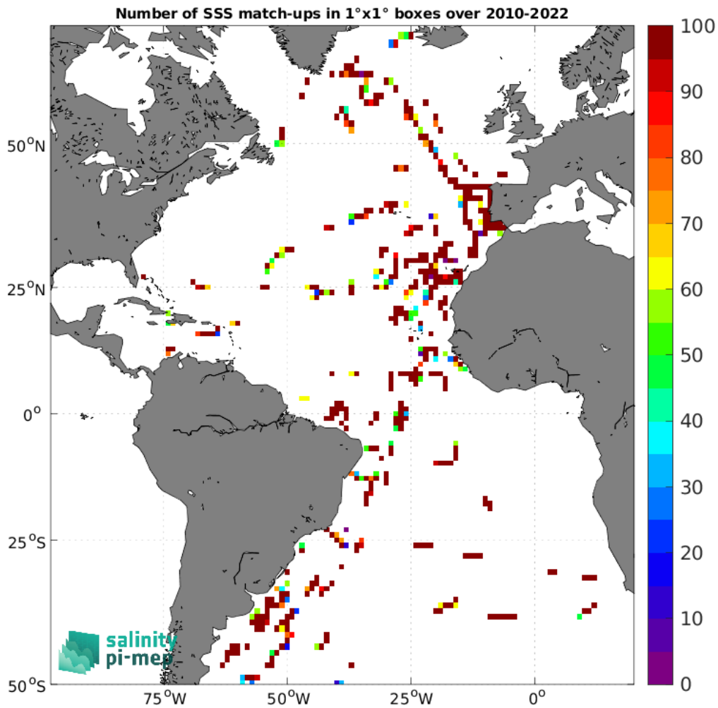
Figure 4: Number of SSS match-ups between TSG (CSIC-UTM) SSS and the SMOS SSS L2Q v331 - 0.25 Deg (CATDS-CPDC) SSS product for the Atlantic Ocean Pi-MEP region over 1°x1° boxes and for the full satellite product period.
