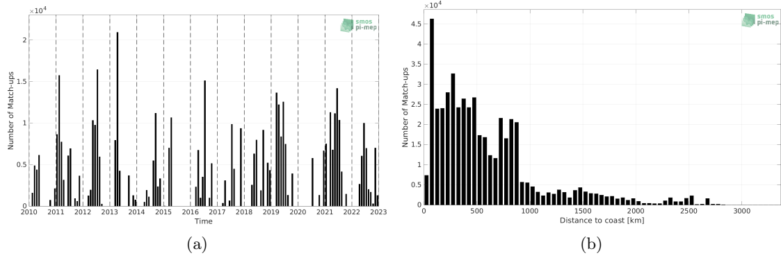
Figure 1: Number of match-ups between TSG (CSIC-UTM) and SMOS SSS L2Q v331 - 0.25 Deg (CATDS-CPDC) SSS as a function of time (a) and as function of the distance to coast (b) over the Atlantic Ocean Pi-MEP region and for the full satellite product period.
