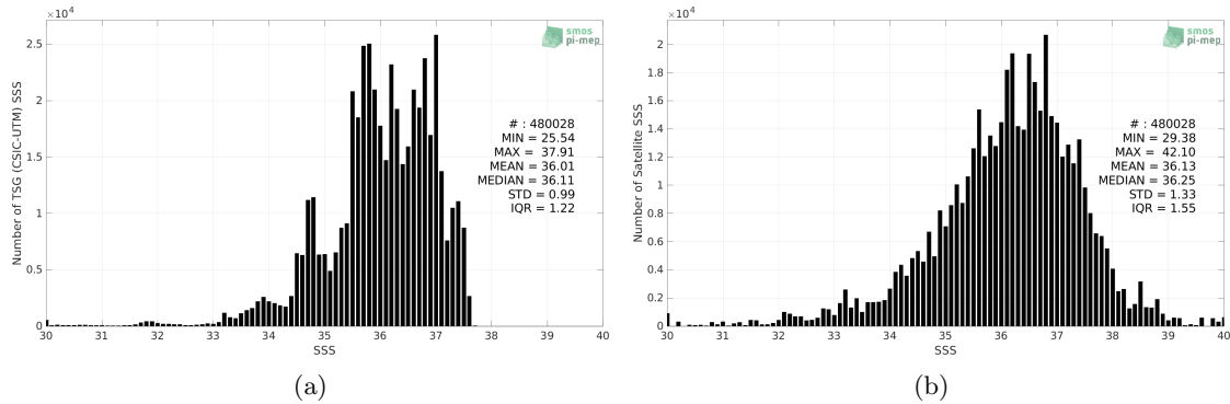
Figure 2: Histograms of SSS from TSG (CSIC-UTM) (a) and SMOS SSS L2Q v331 - 0.25 Deg (CATDS-CPDC) (b) considering all match-up pairs per bins of 0.1 over the Atlantic Ocean Pi-MEP region and for the full satellite product period.
