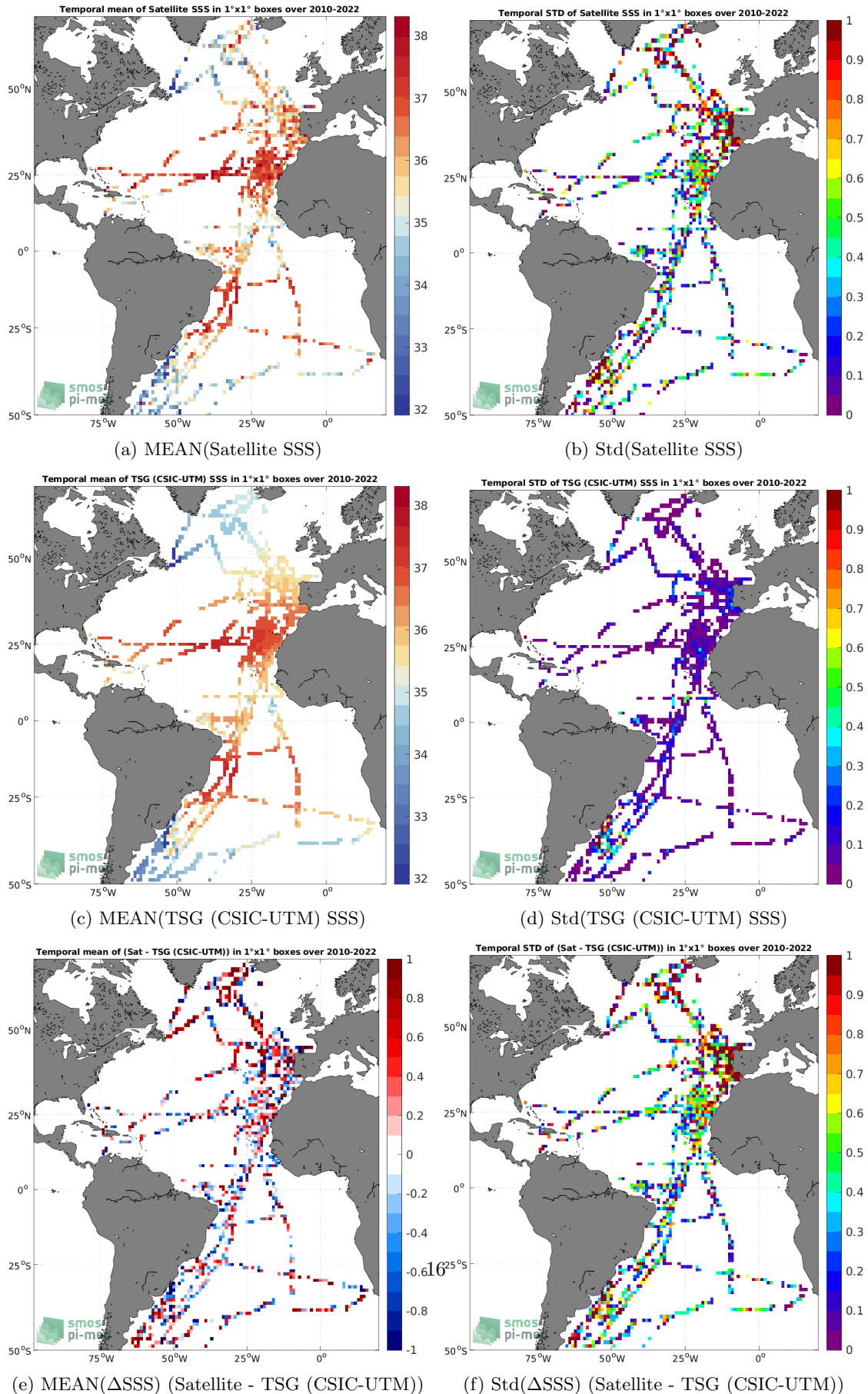
Figure 6: Temporal mean (left) and Std (right) of SSS from SMOS SSS L2Q v331 - 0.25 Deg (CATDS-CPDC) (top), TSG (CSIC-UTM) (middle), and of \Delta SSS (Satellite - TSG (CSIC-UTM)). Only match-up pairs are used to generate these maps.
